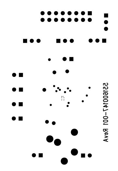
Figure 46. Bottom Silkscreen
