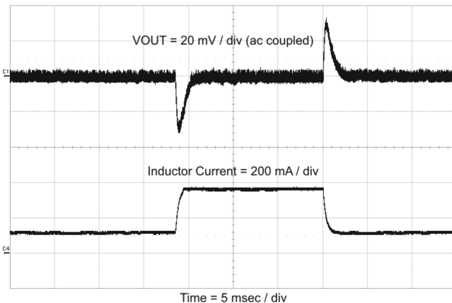
Figure 52. Load Transient
