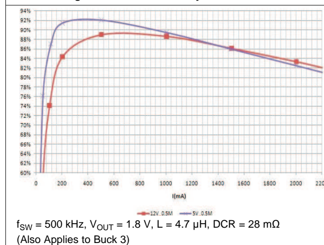
Figure 5. BUCK2 Efficiency
