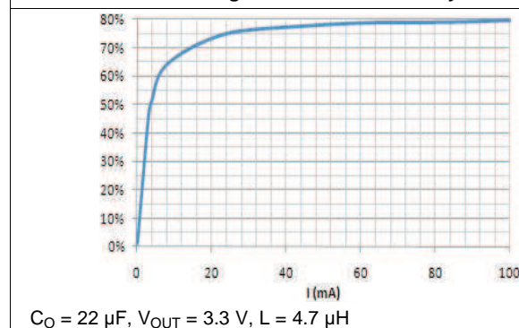
Figure 1. BUCK1 Efficiency
