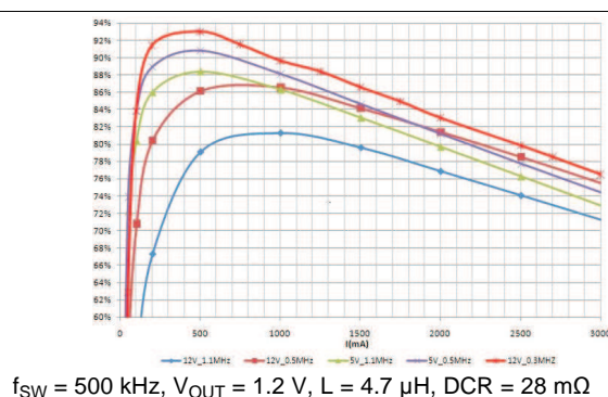
Figure 2. BUCK1 Efficiency
