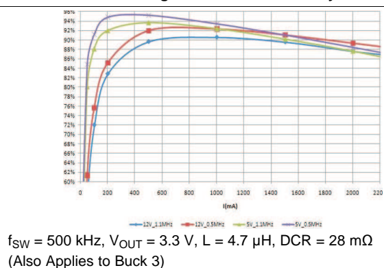
Figure 4. BUCK2 Efficiency
