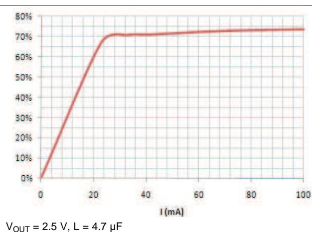
Figure 4. BUCK2 Efficiency
