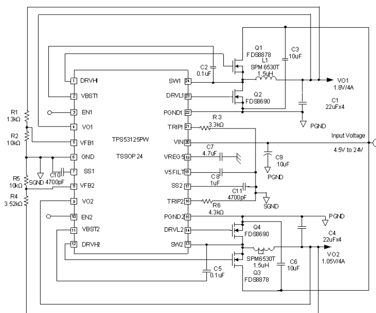
Figure 2. TSSOP
