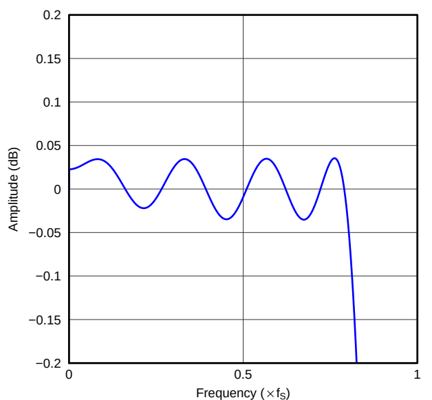
Figure 58. Asymmetric x4 Interpolation Filter Passband Ripple, Dual Rate
