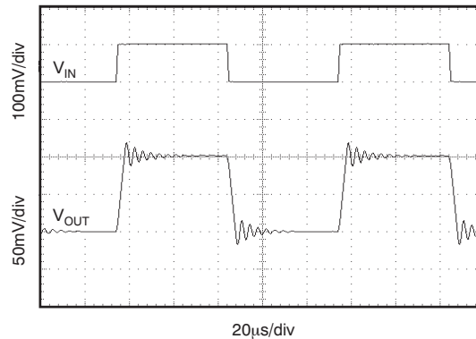
Figure 44. OPA827 Driving 2.2-μF Ceramic Capacitor
