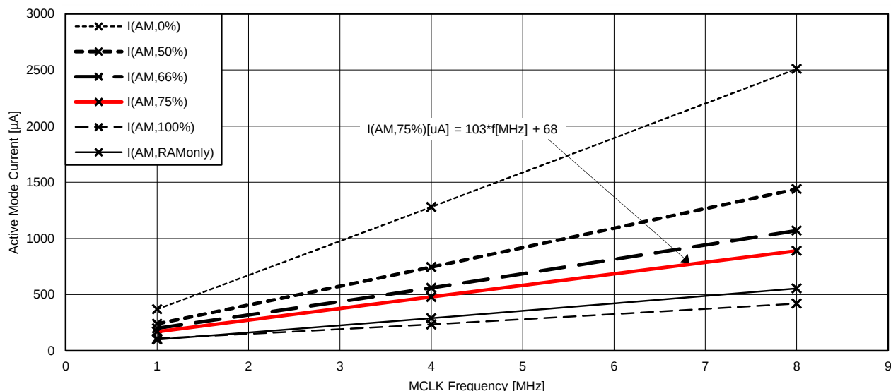
Figure 5-1. Typical Active Mode Supply Currents vs MCLK frequency, No Wait States
