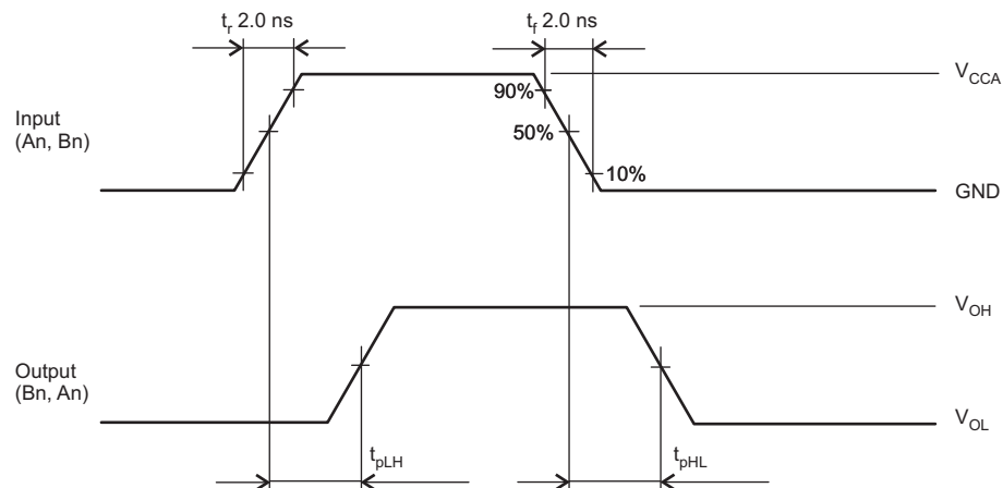
Figure 7. t_{PLH} , t_{PHL}
