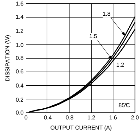
Figure 14. Dissipation 4.5-V Input at 85°C
