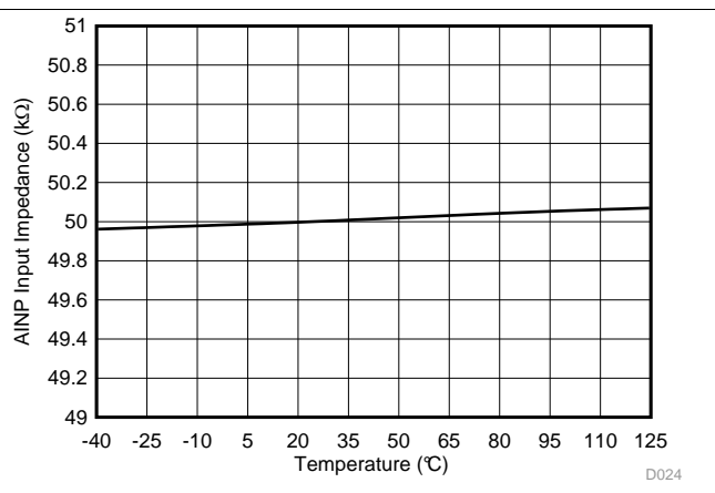
Figure 24. Shunt Sense Amplifier AINP Input Impedance vs Temperature
