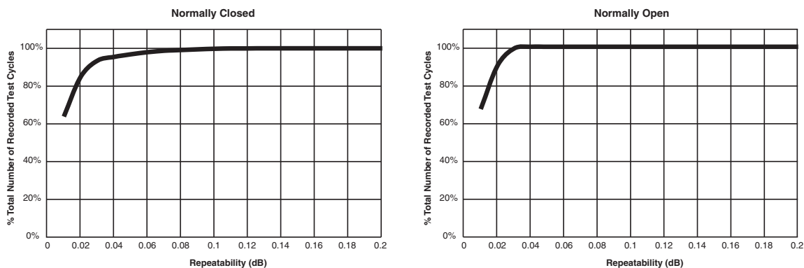
REPEATABILITY CHARACTERISTICS GRF300 RELAYS
