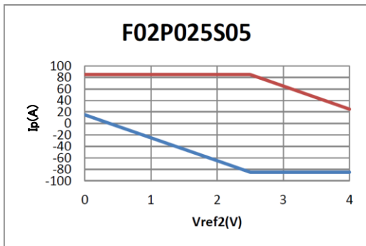
Upper limit: I_p = 85 ( V_{ref2}=0...2.5V ) I_p = -40 \times V_{ref2} + 185 ( V_{ref2}=2.5...4V ) Lower limit: I_p = -40 \times V_{ref2} + 15 ( V_{ref2}=0...2.5V ) I_p = -85 ( V_{ref2}=2.5...4V )
