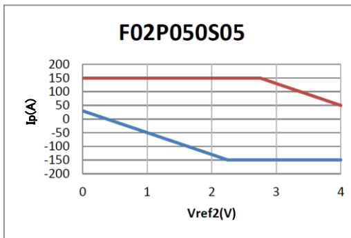
Upper limit: I_p = 150 ( V_{ref2}=0...2.75V ) I_p = -80 \times V_{ref2} + 370 ( V_{ref2}=2.75...4V ) Lower limit: I_p = -80 \times V_{ref2} + 30 ( V_{ref2}=0...2.25V ) I_p = -150 ( V_{ref2}=2.25...4V )
