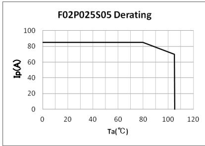
Figure 5 : Ip vs Ta for F02P025S05
