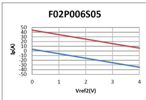
Upper limit: I_p = -9.6 \times V_{ref2} + 44.4 ( V_{ref2}=0...4V ) Lower limit: I_p = -9.6 \times V_{ref2} + 3.6 ( V_{ref2}=0...4V )
