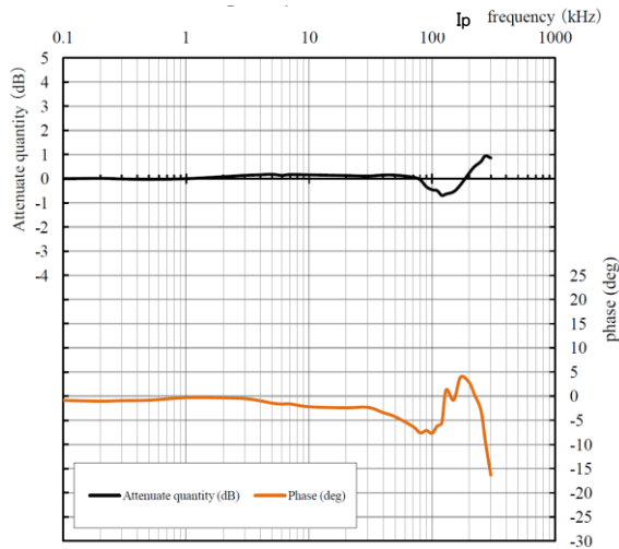
Figure 2: Frequency response curve ex) F02P025S05
