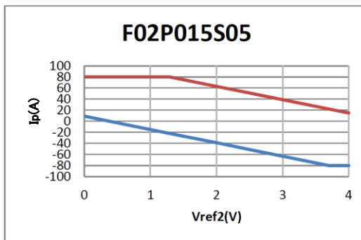
Upper limit: I_p = 80 ( V_{ref2}=0...1.29V ) I_p = -24 \times V_{ref2} + 111 ( V_{ref2}=1.29...4V ) Lower limit: I_p = -24 \times V_{ref2} + 9 ( V_{ref2}=0...3.7V ) I_p = -80 ( V_{ref2}=3.7...4V )
