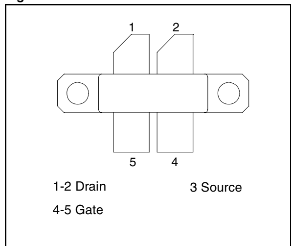
Figure 1. Pin connections
