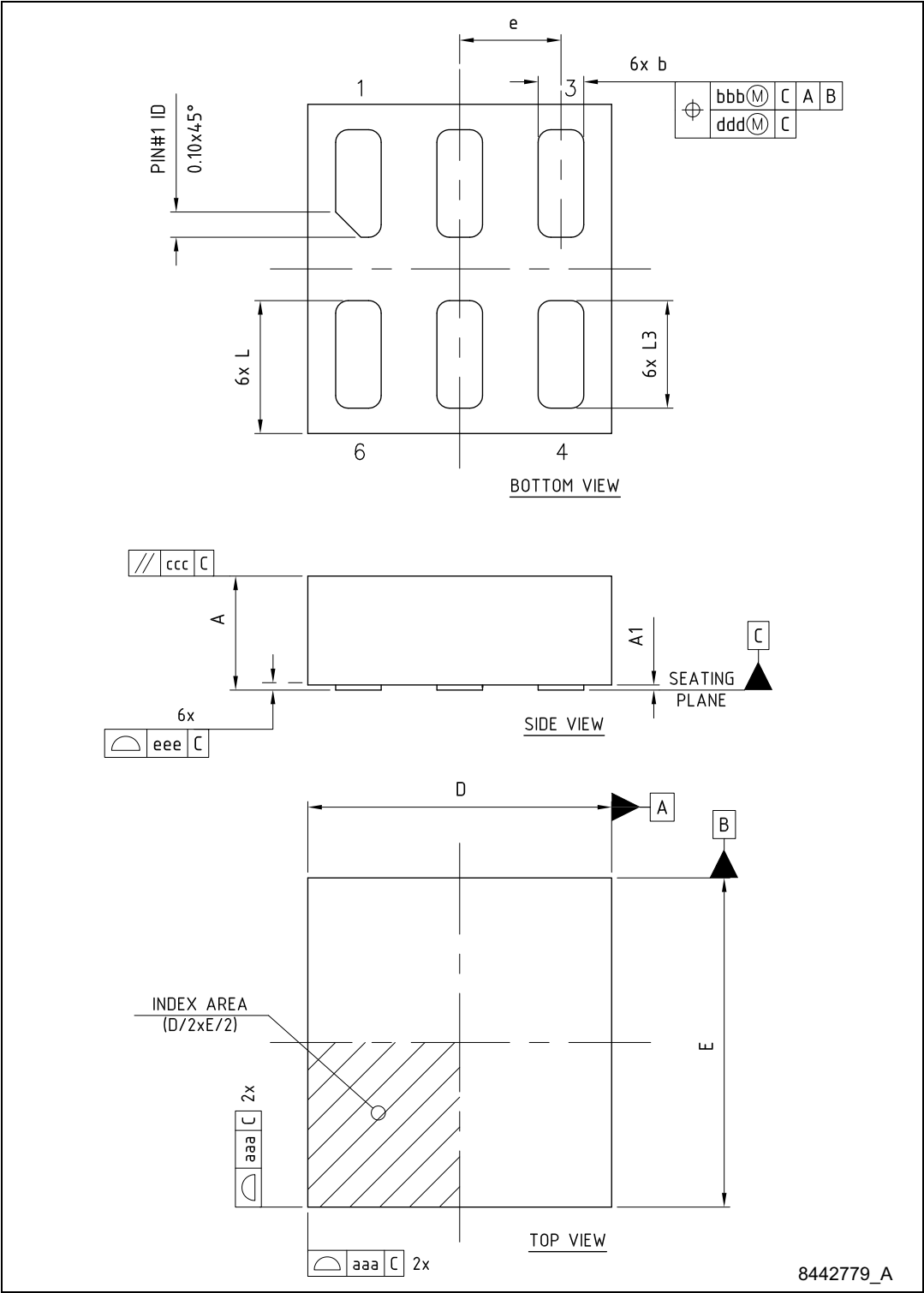
Figure 34. DFN6-1.2x1.3 drawings
