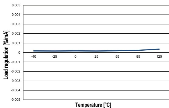
Figure 13. Load regulation vs. temperature ( V_{OUT}=V_{ADJ} )
