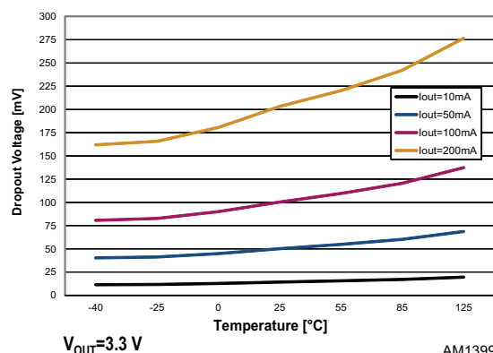
Figure 15. Dropout voltage vs. temperature
