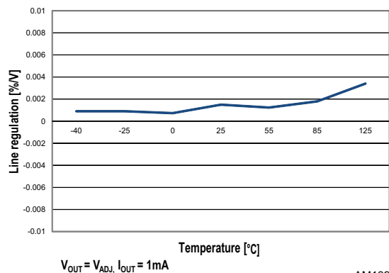
Figure 11. Line regulation vs. temperature ( V_{OUT}=V_{ADJ} )
