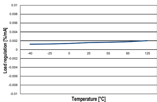
Figure 12. Load regulation vs. temperature ( V_{OUT}=3.3\text{ V} )
