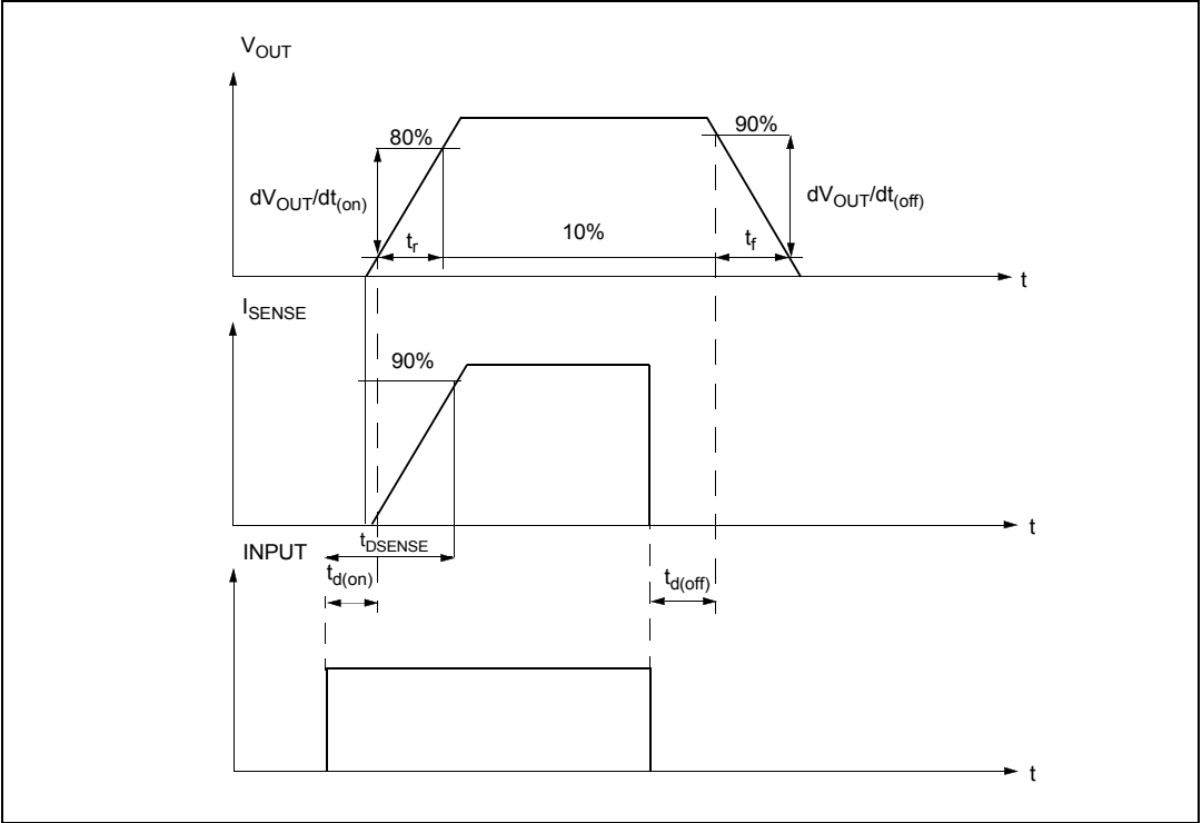
Figure 4. Switching characteristics (resistive load R_L = 6.5 \Omega )
