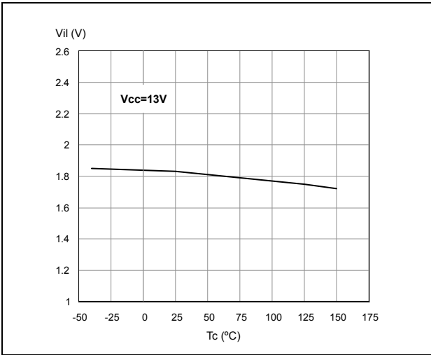
Figure 11. Input low level
