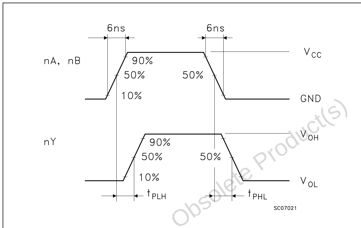
WAVEFORM 1: PROPAGATION DELAY TIME ( f=1\text{MHz} ; 50% duty cycle)
