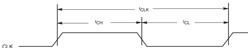
Figure 10.6 CLK Characterization
