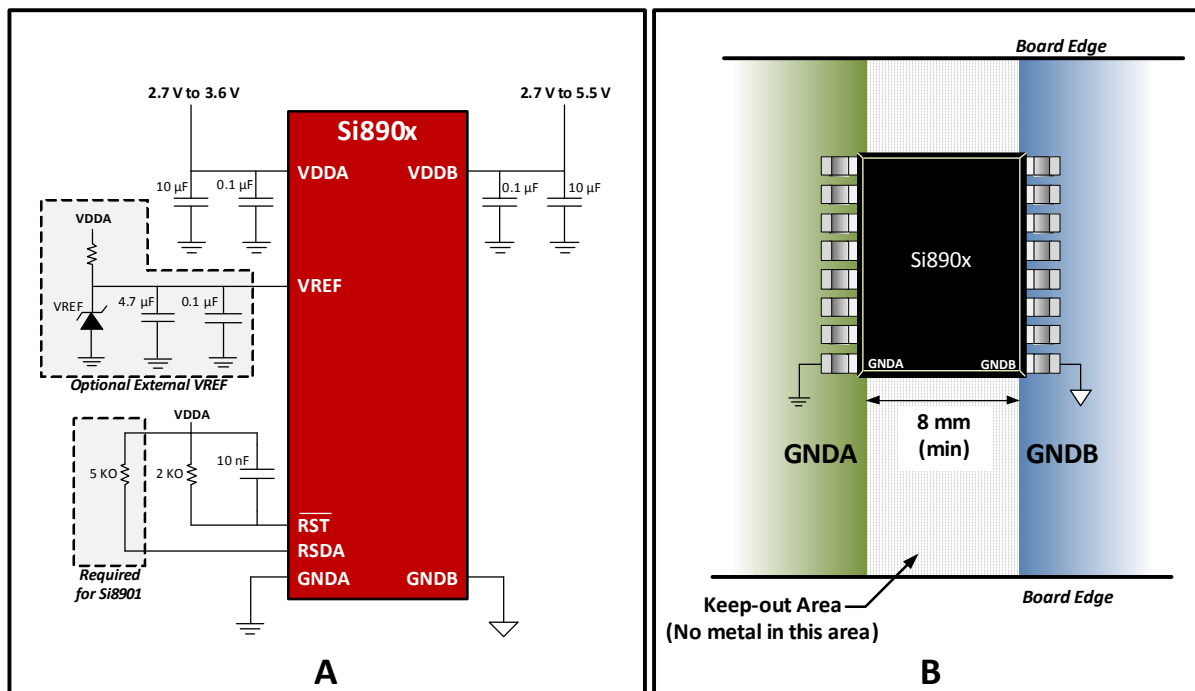
Figure 14. Si890x Installation
