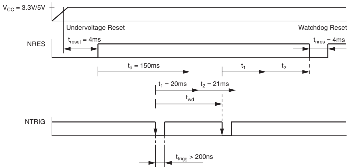
Figure 2-2. Timing Sequence with R3 = 51kΩ at the Atmel ATA6622/24/26
