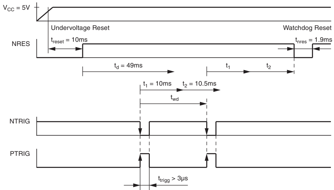
Figure 2-1. Timing Sequence with R3 = 51kΩ at the Atmel ATA6621
