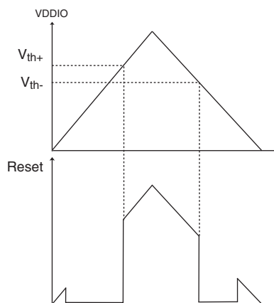
Figure 40-3. Zero-Power-on Reset Characteristics
