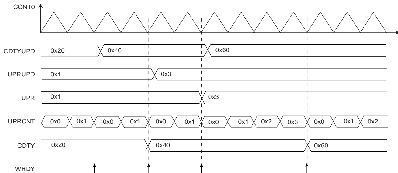
Figure 35-11. Method 2 (UPDM=1)
