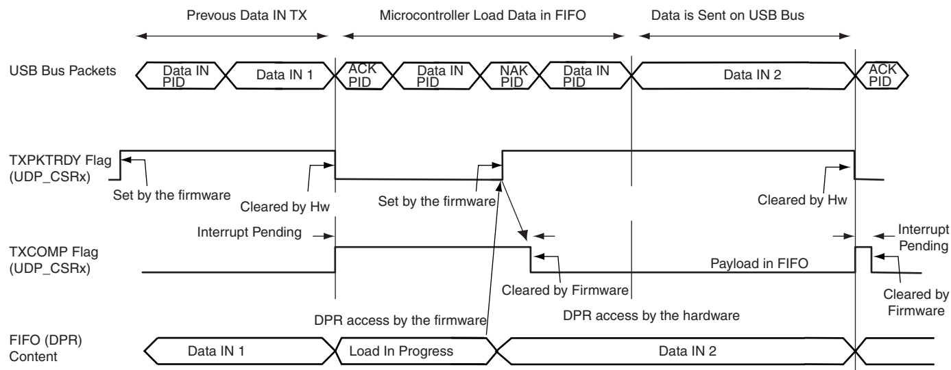
Figure 36-7. Data IN Transfer for Non Ping-pong Endpoint
