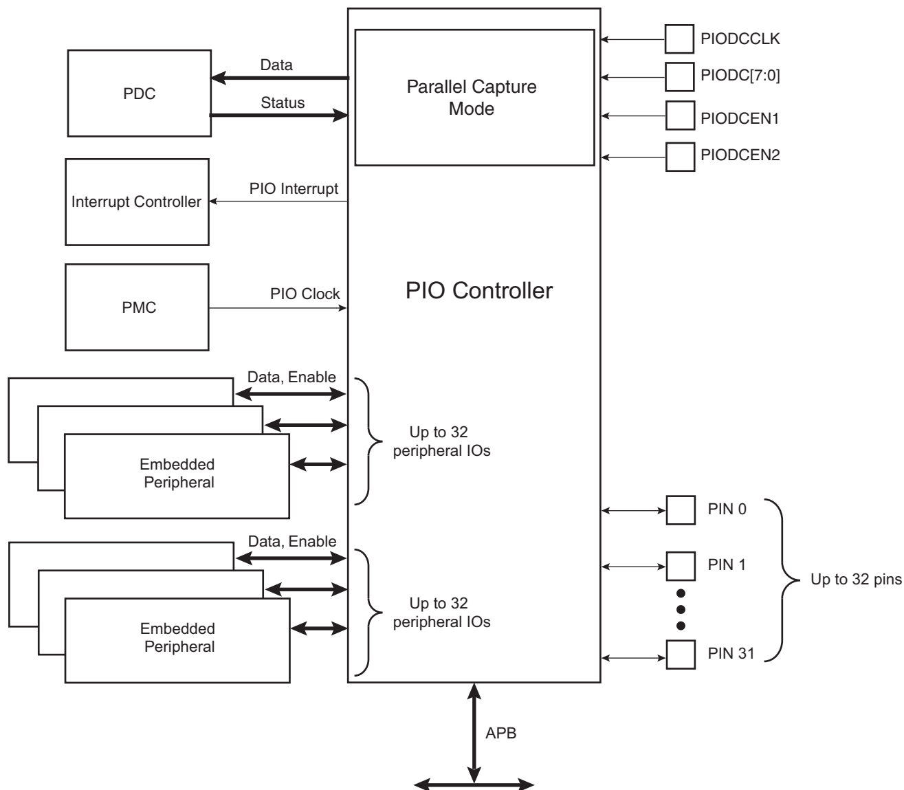
Figure 27-1. Block Diagram
