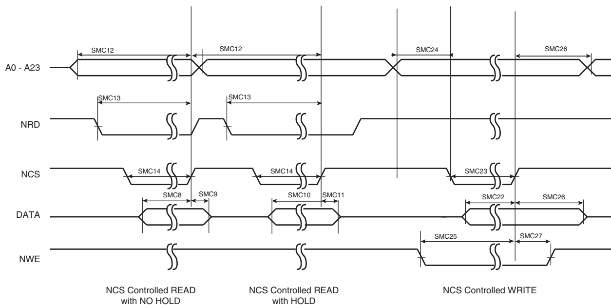
Figure 40-29. SMC Timings - NCS Controlled Read and Write
