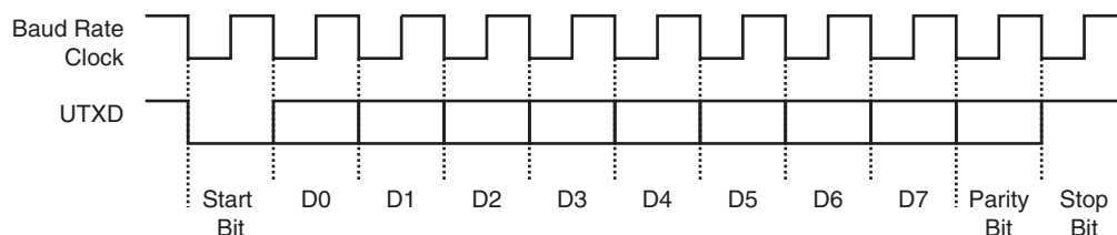
Figure 31-9. Character Transmission
