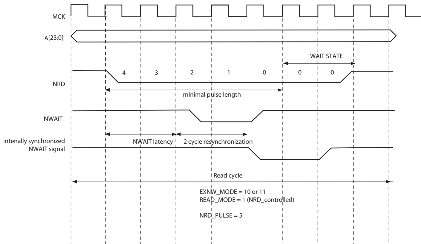
Figure 23-27. NWAIT Latency
