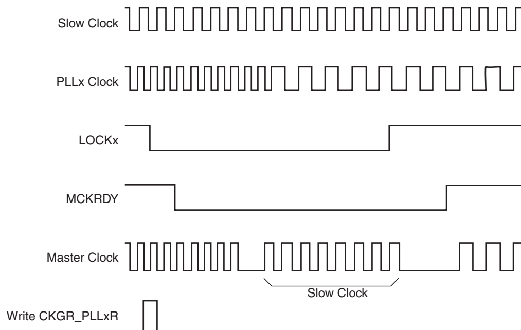
Figure 25-12. Change PLLx Programming
