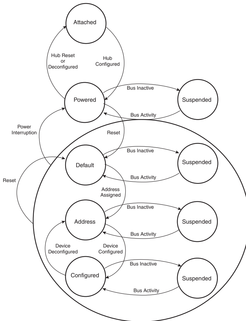
Figure 36-15. USB Device State Diagram
