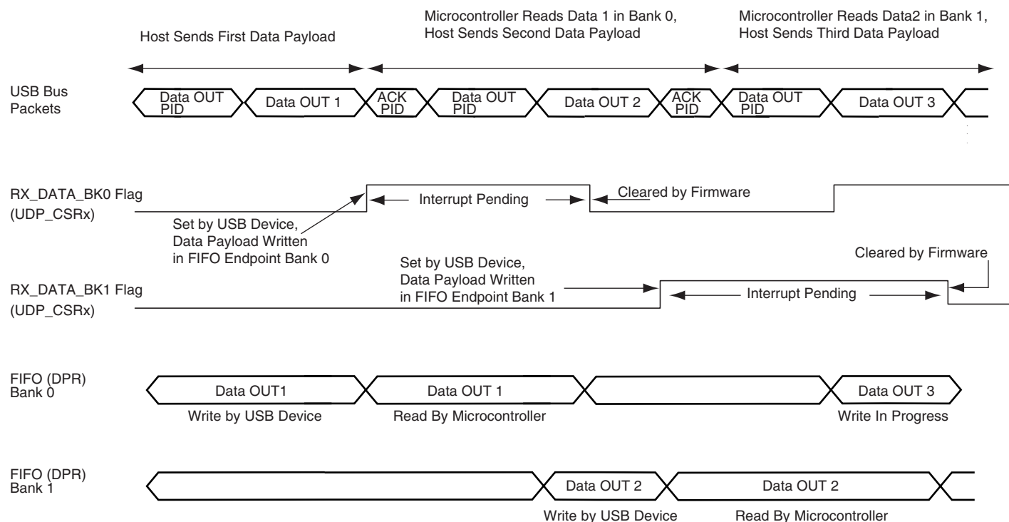
Figure 36-12. Data OUT Transfer for Ping-pong Endpoint
