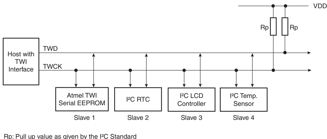
Figure 29-2. Application Block Diagram
