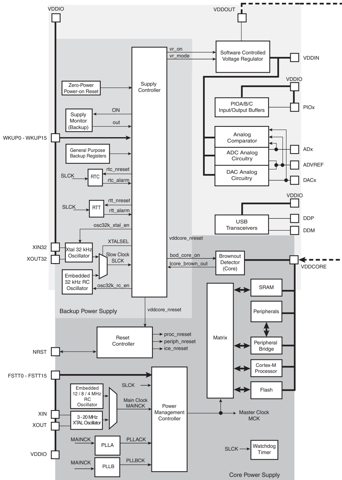
Figure 16-1. Supply Controller Block Diagram
