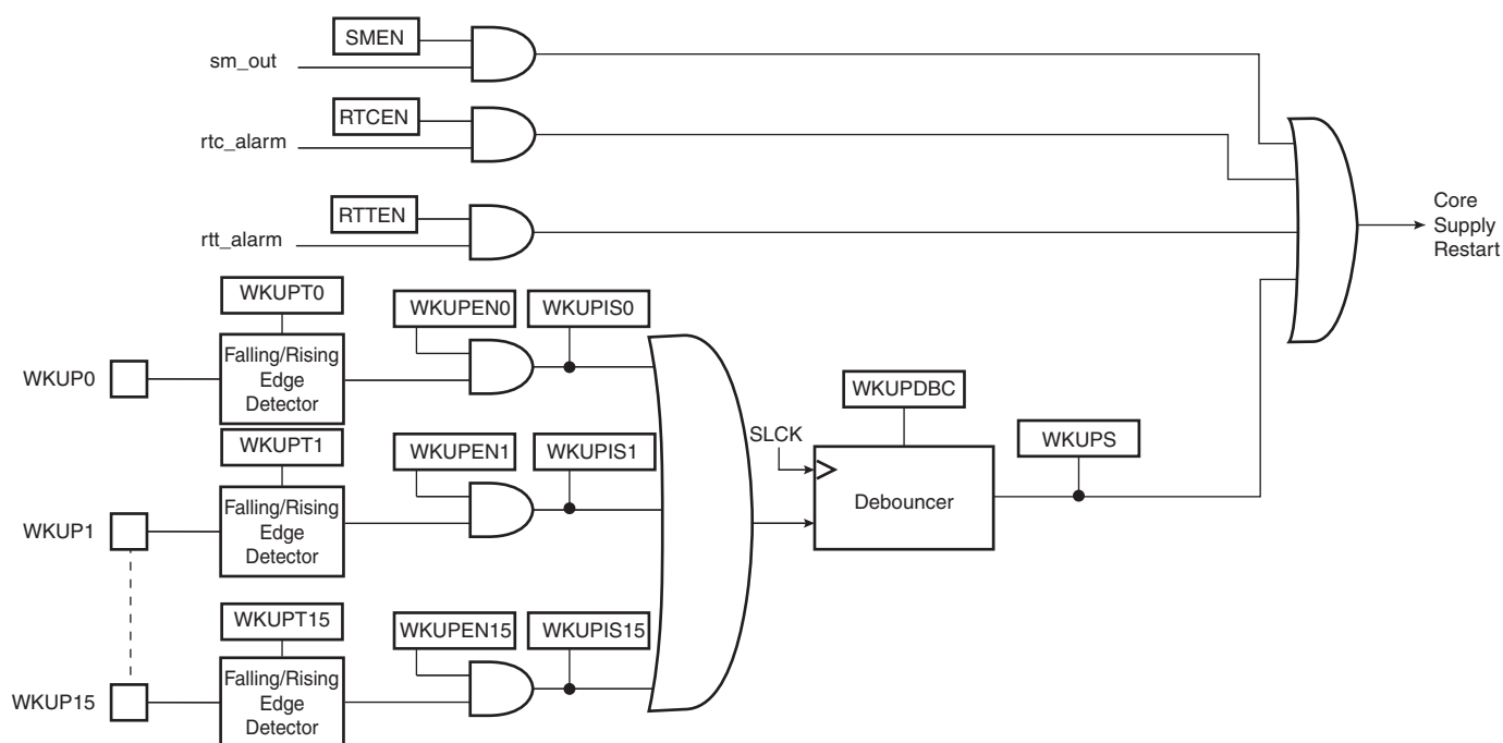
Figure 5-4. Wake-up Source
