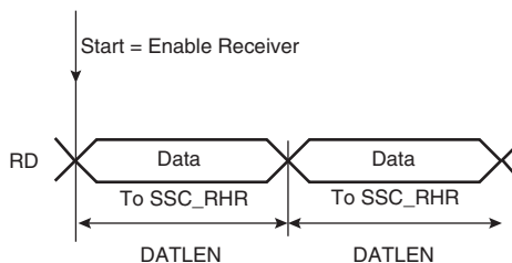
Figure 28-15. Receive Frame Format in Continuous Mode
