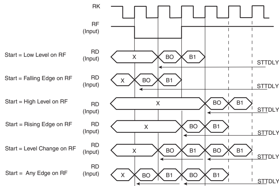
Figure 28-11. Receive Pulse/Edge Start Modes
