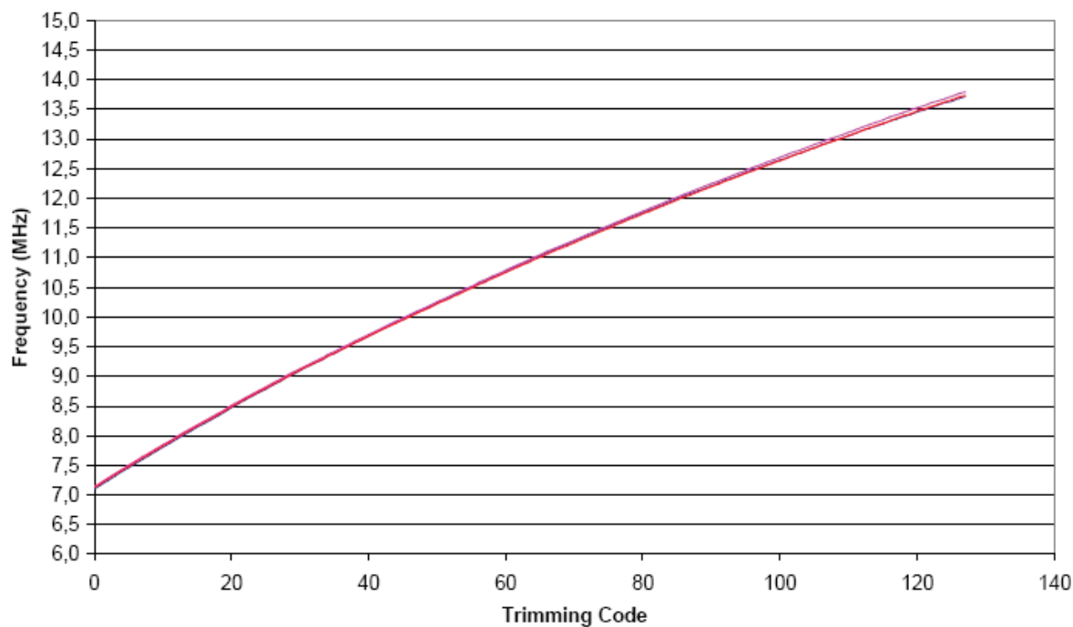
Figure 40-13. RC 12 MHz trimming
