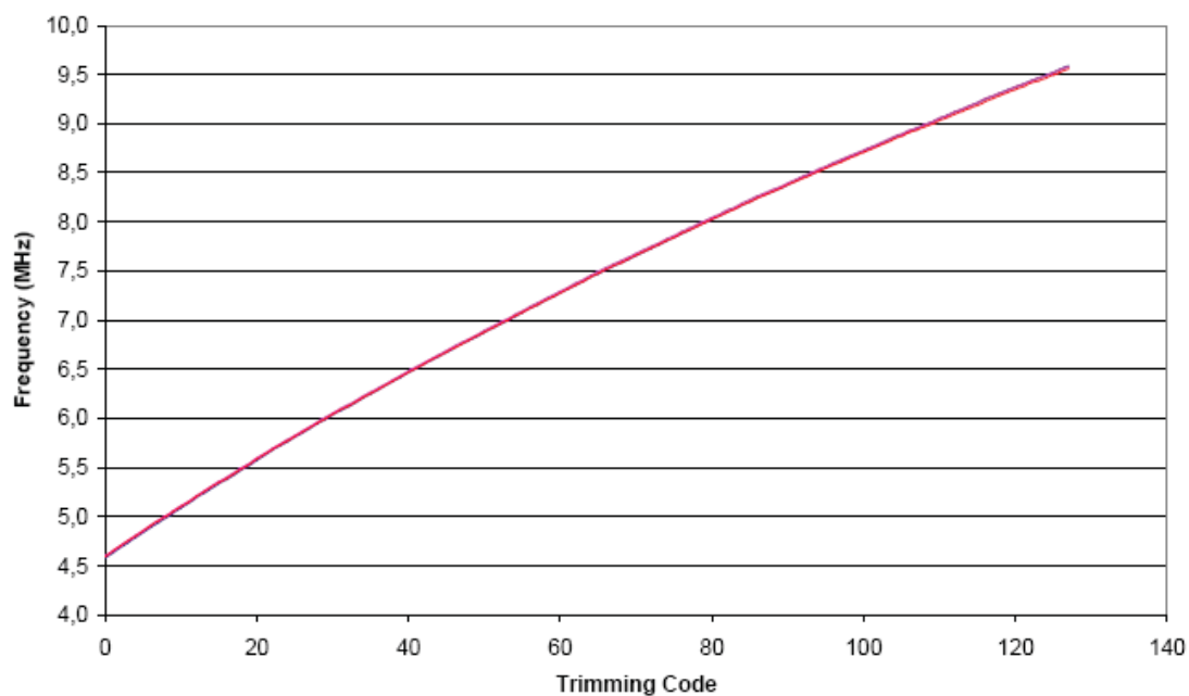
Figure 40-12. RC 8 MHz trimming
