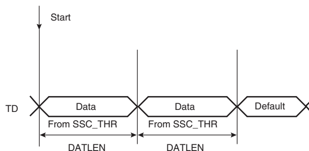
Figure 28-14. Transmit Frame Format in Continuous Mode
