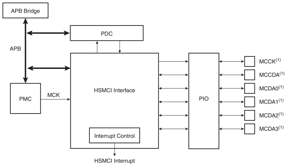
Figure 34-1. Block Diagram
