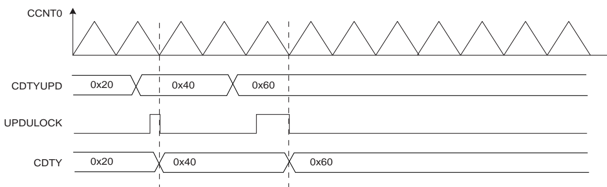
Figure 35-10. Method 1 (UPDM = 0)
