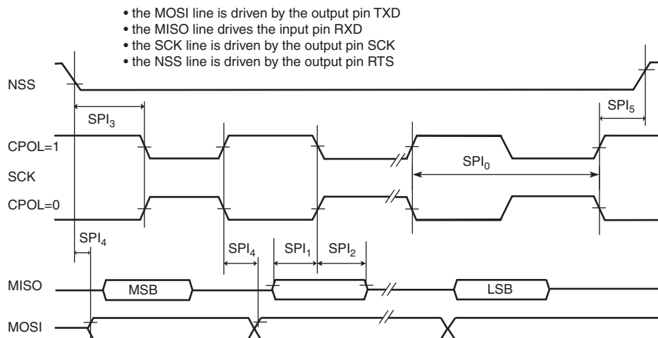
Figure 40-31. USART SPI Master Mode
