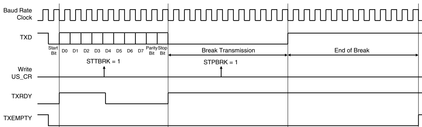
Figure 32-26. Break Transmission
