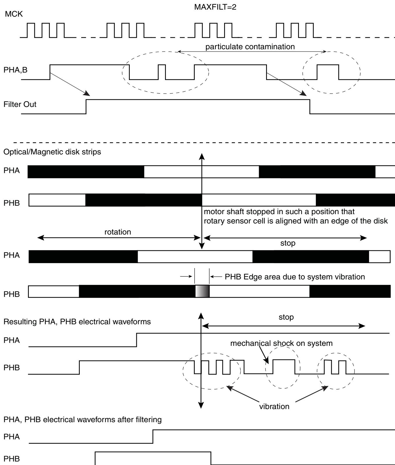
Figure 33-17. Filtering Examples
