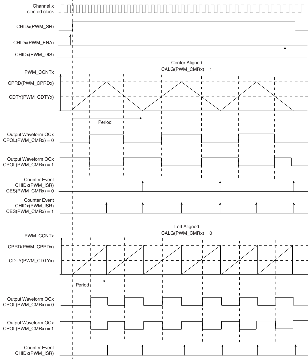
Figure 35-5. Waveform Properties
