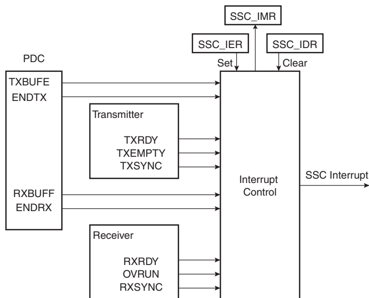
Figure 28-16. Interrupt Block Diagram
