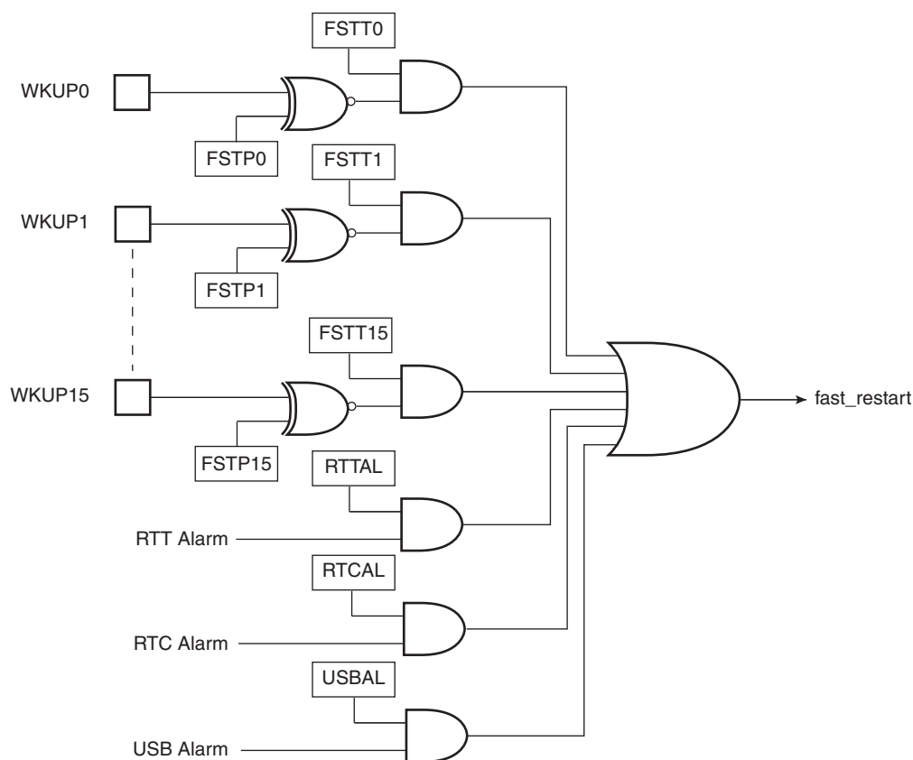
Figure 25-9. Fast Startup Circuitry
