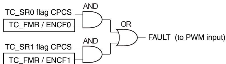
Figure 33-21. Fault Output Generation
