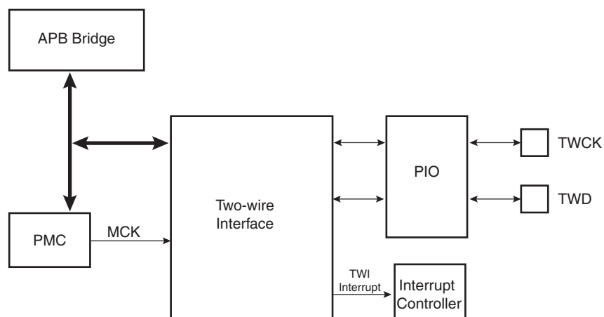
Figure 29-1. Block Diagram
