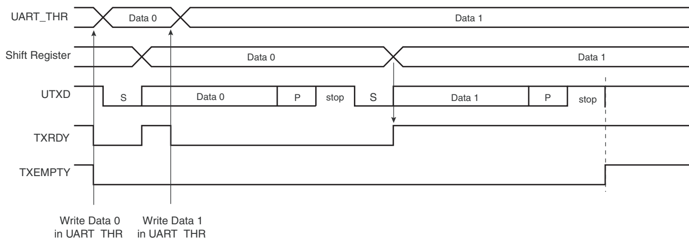
Figure 31-10. Transmitter Control
