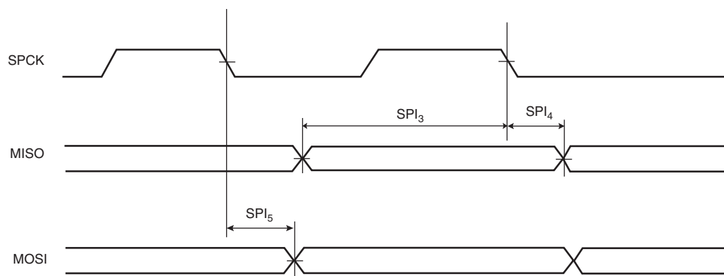
Figure 40-17. SPI Master Mode with (CPOL = 0 and NCPHA=1) or (CPOL=1 and NCPHA= 0)
