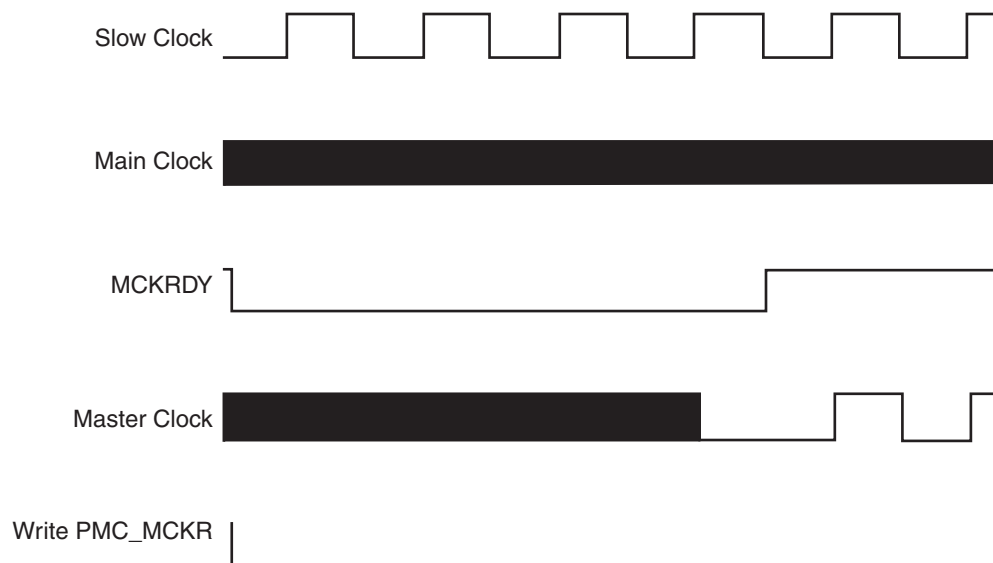
Figure 25-11. Switch Master Clock from Main Clock to Slow Clock
