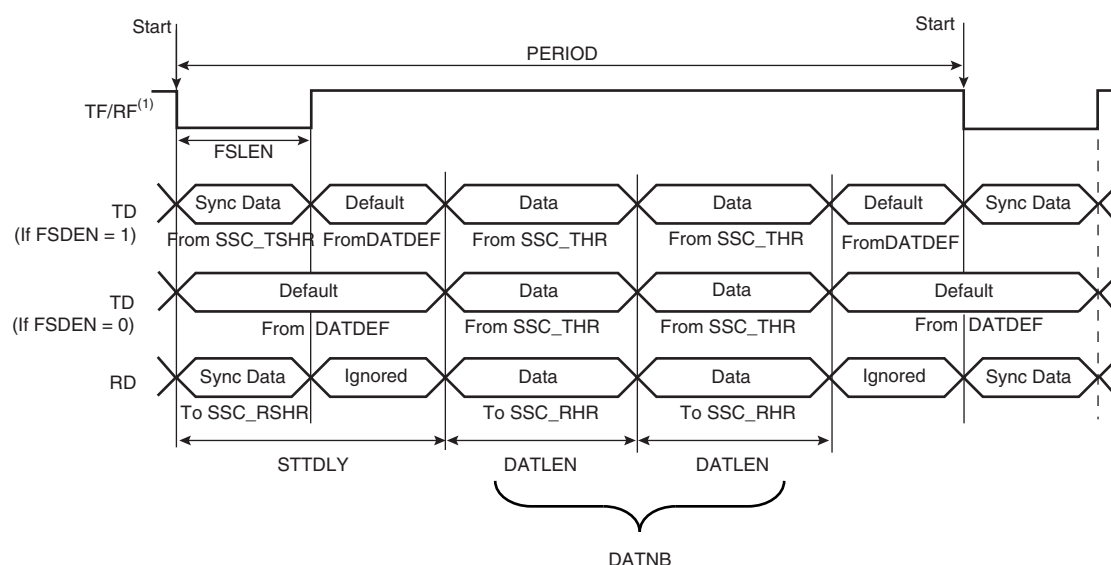
Figure 28-13. Transmit and Receive Frame Format in Edge/Pulse Start Modes
