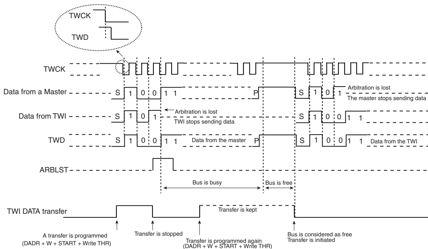
Figure 29-22. Arbitration Cases
