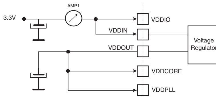
Figure 40-4. Measurement Setup
