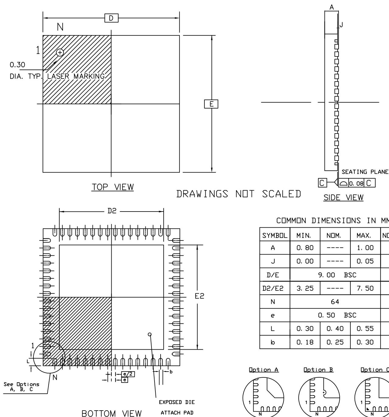
Figure 41-4. 64-pad QFN Package Drawing
