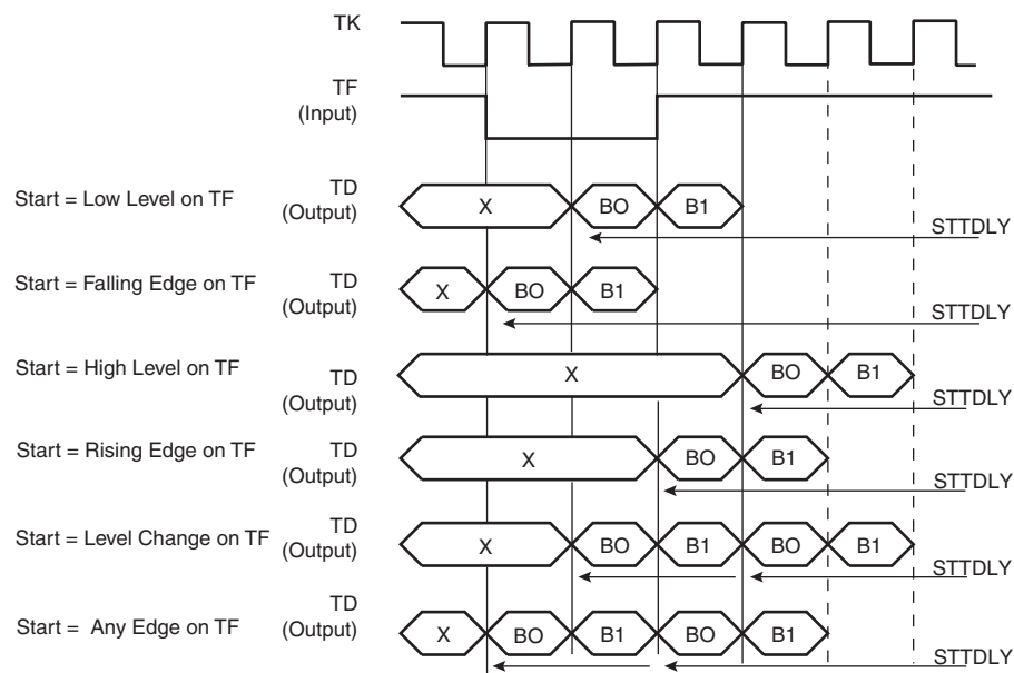
Figure 28-10. Transmit Start Mode
