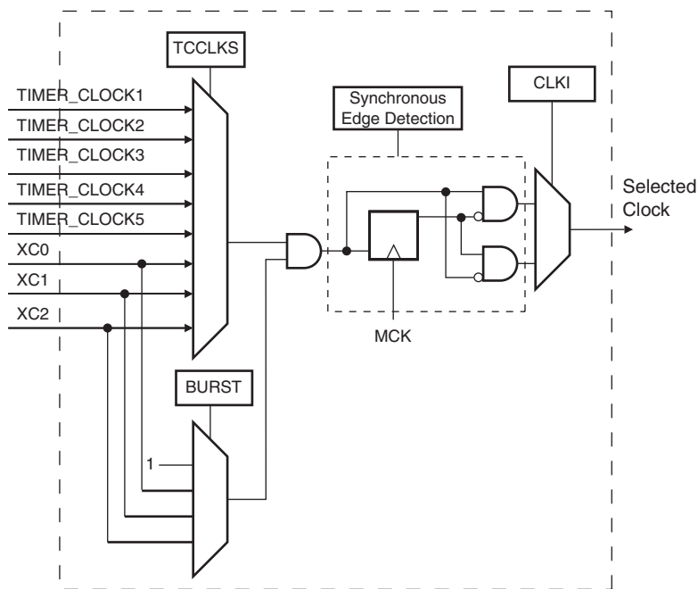
Figure 33-3. Clock Selection
