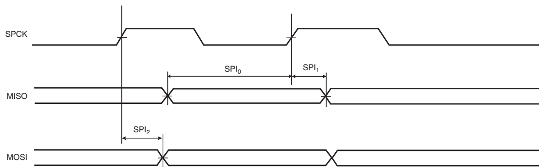
Figure 40-16. SPI Master Mode with (CPOL= NCPHA = 0) or (CPOL= NCPHA= 1)
