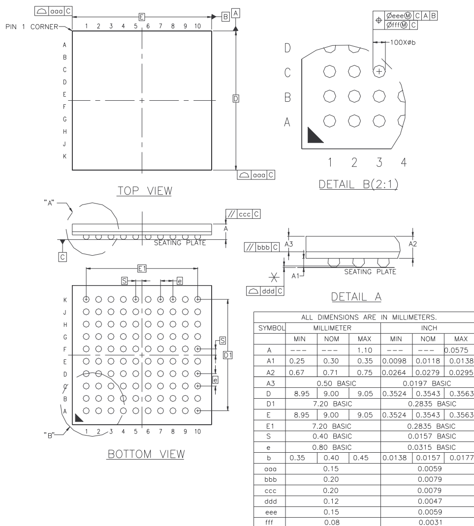
Figure 41-2. 100-ball LFBGA Package Drawing
