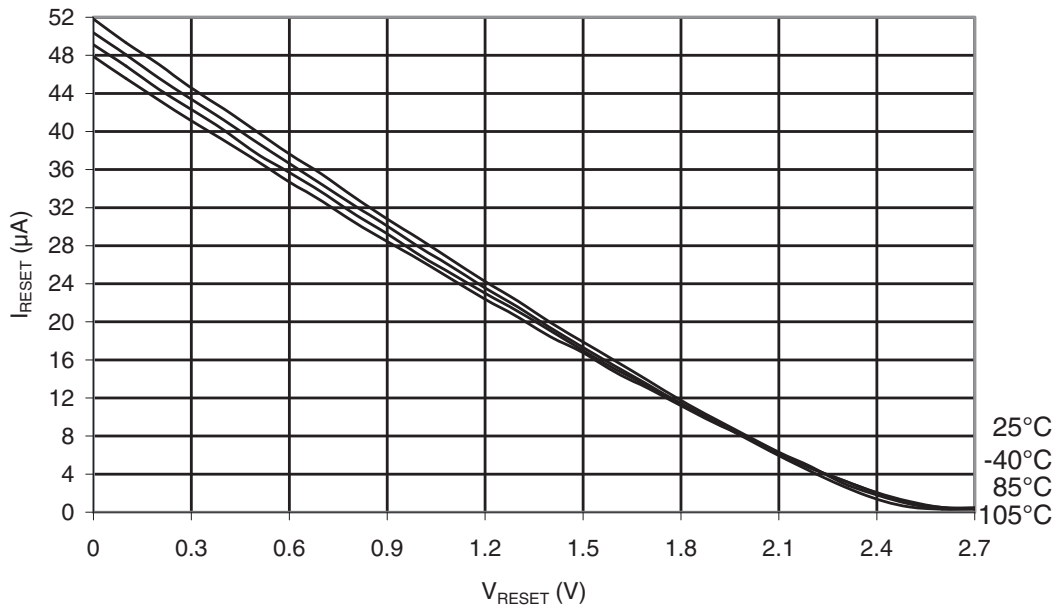
Figure 32-19. ATmega48PA: Reset Pull-up Resistor Current vs. Reset Pin Voltage ( V_{CC} = 2.7V )
