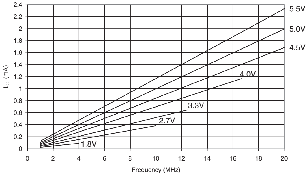
Figure 32-45. ATmega48PA: Reset Supply Current vs. Frequency (1MHz- 20MHz)
