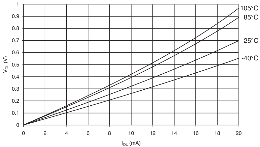
Figure 32-21. ATmega48PA: I/O Pin Output Voltage vs. Sink Current ( V_{CC} = 3V )
