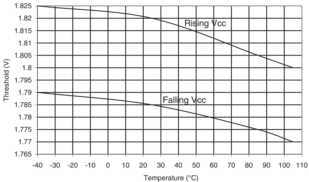
Figure 32-31. ATmega48PA: BOD Thresholds vs. Temperature (BODLEVEL is 1.8V)
