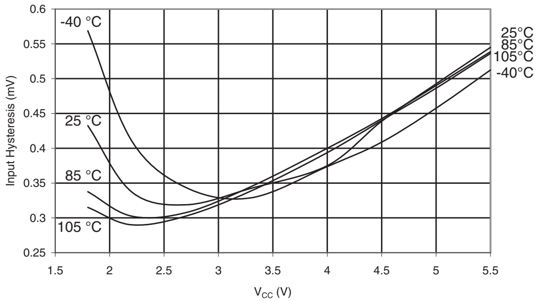
Figure 32-27. ATmega48PA: I/O Pin Input Hysteresis vs. V_{CC}
