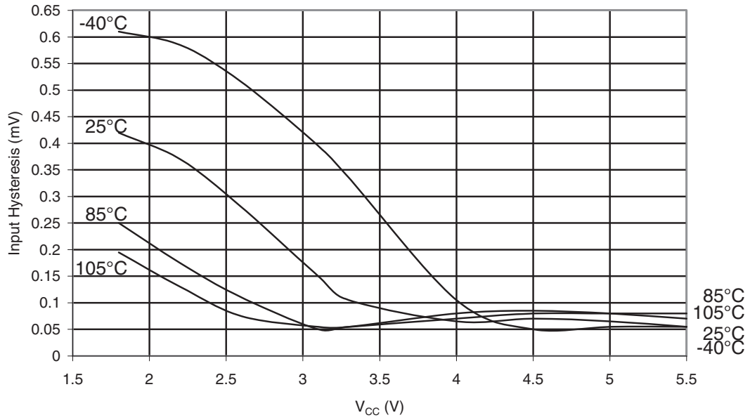
Figure 32-30. ATmega48PA: Reset Pin Input Hysteresis vs. V_{CC}
