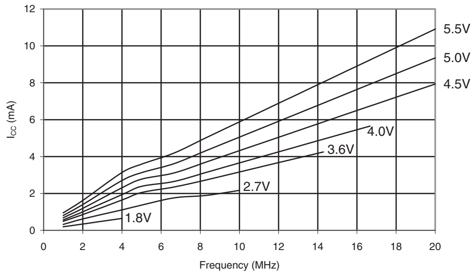
Figure 31-238. ATmega168PA: Active Supply Current vs. Frequency (1-20MHz)
