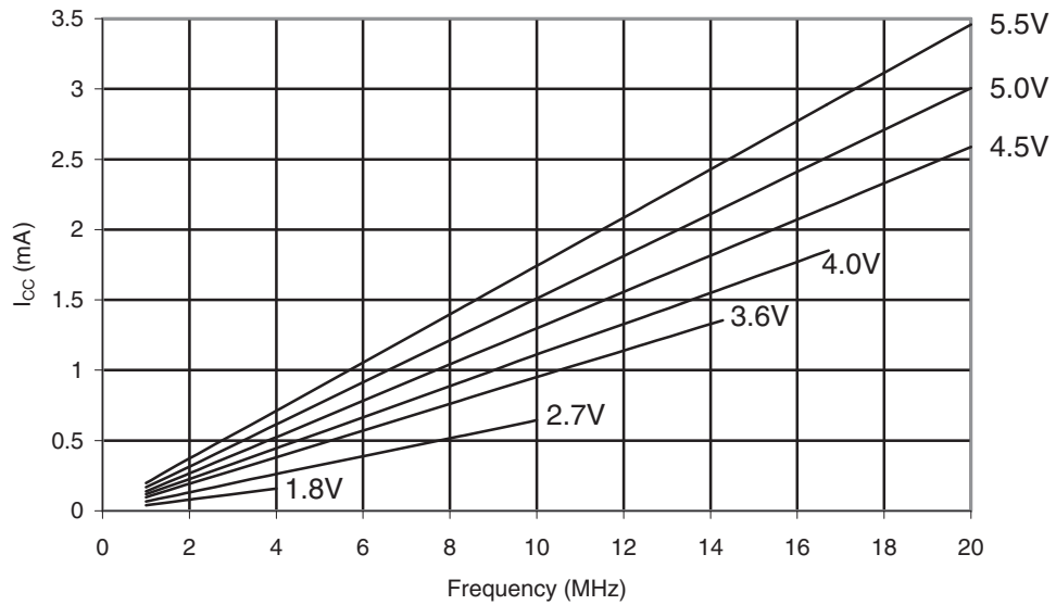
Figure 31-333. ATmega328P: Active Supply Current vs. Frequency (1-20MHz)
