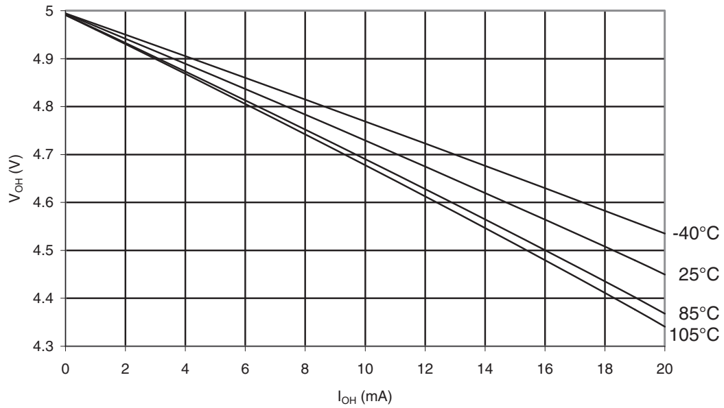
Figure 32-24. ATmega48PA: I/O Pin Output Voltage vs. Source Current ( V_{CC} = 5V )
