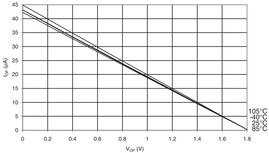
Figure 32-15. ATmega48PA: I/O Pin Pull-up Resistor Current vs. Input Voltage ( V_{CC} = 1.8V )
