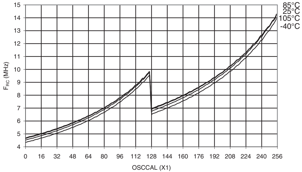
Figure 32-38. ATmega48PA: Calibrated 8MHz RC Oscillator Frequency vs. OSCCAL Value
