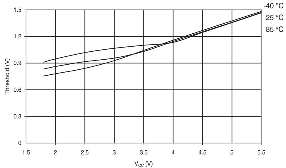
Figure 31-122. ATmega88A: Reset Input Threshold Voltage vs. V_{CC} ( V_{IH} , I/O Pin read as '1')
