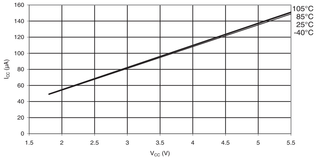
Figure 31-185. ATmega88PA: Brownout Detector Current vs. V_{CC}
