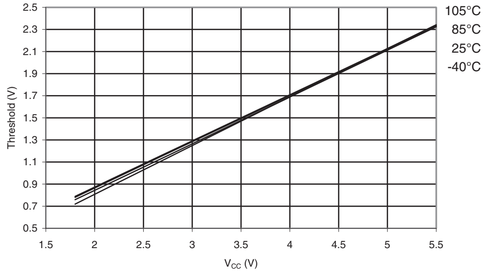
Figure 31-360. ATmega328P: Reset Input Threshold Voltage vs. V_{CC} ( V_{IL} , I/O Pin read as '0')
