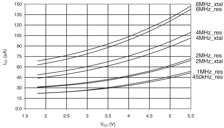
Figure 32-14. ATmega48PA: Standby Supply Current vs. V CC (Watchdog Timer Disabled)
