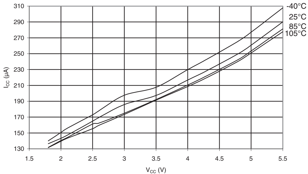
Figure 32-39. ATmega48PA: ADC Current vs. V_{CC} (AREF = AV_{CC} )
