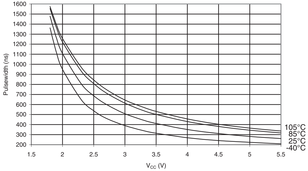
Figure 32-46. ATmega48PA: Minimum Reset Pulse width vs. V_{CC}
