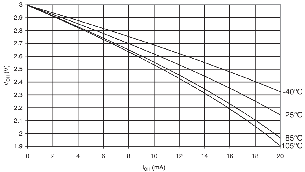
Figure 32-23. ATmega48PA: I/O Pin Output Voltage vs. Source Current ( V_{CC} = 3V )
