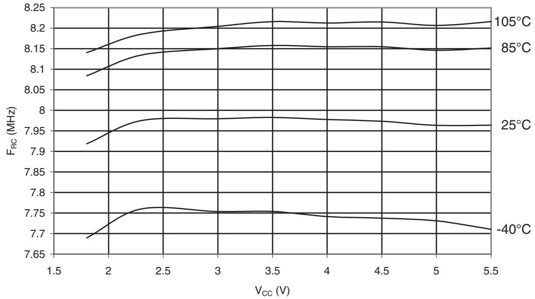
Figure 32-36. ATmega48PA: Calibrated 8MHz RC Oscillator Frequency vs. V_{CC}
