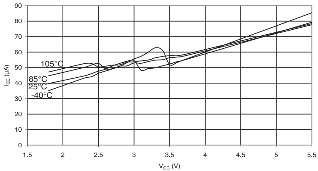
Figure 31-183. ATmega88PA: Analog Comparator Current vs. V_{CC}
