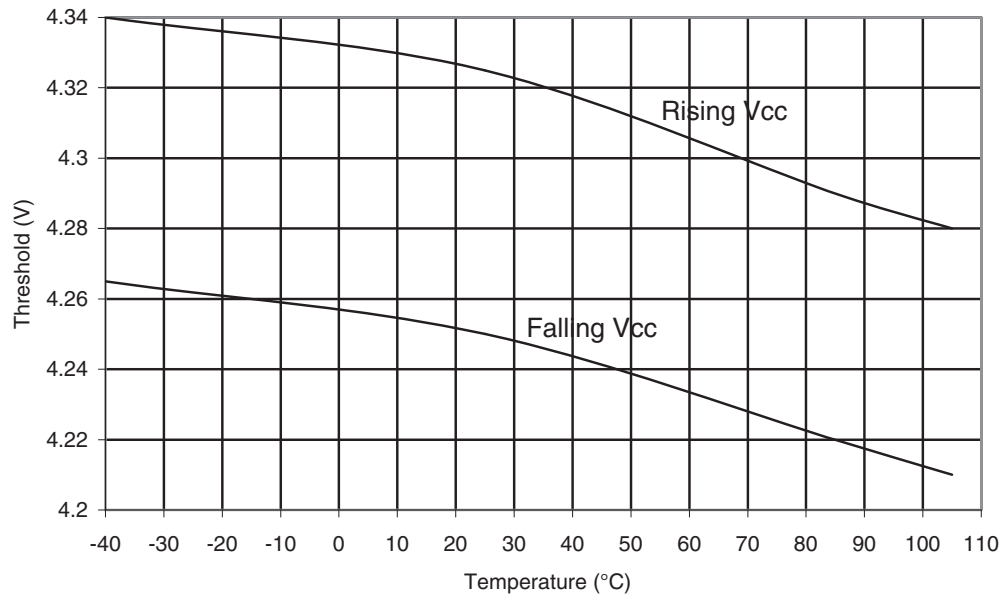
Figure 32-33. ATmega48PA: BOD Thresholds vs. Temperature (BODLEVEL is 4.3V)
