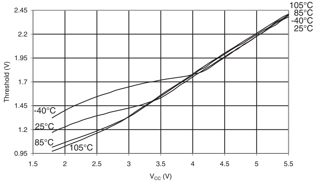
Figure 32-29. ATmega48PA: Reset Input Threshold Voltage vs. V_{CC} ( V_{IL} , I/O Pin read as '0')
