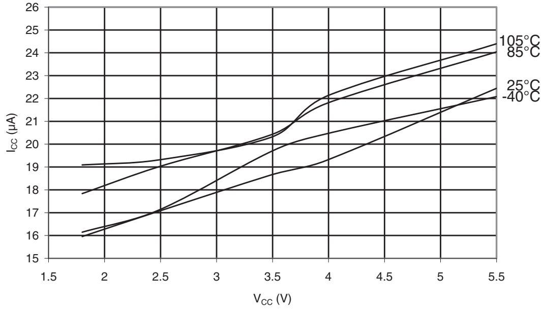
Figure 32-43. ATmega48PA: Programming Current vs. V_{CC}
