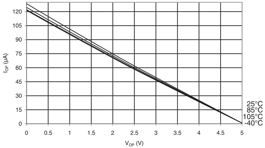
Figure 32-17. ATmega48PA: I/O Pin Pull-up Resistor Current vs. Input Voltage ( V_{CC} = 5V )
