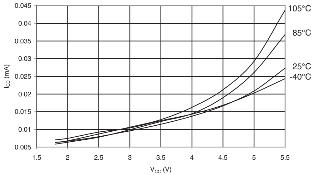
Figure 31-244. ATmega168PA: Idle Supply Current vs. V_{CC} (Internal RC Oscillator, 128kHz)
