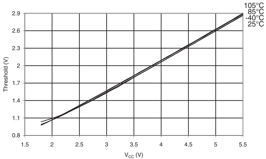
Figure 32-25. ATmega48PA: I/O Pin Input Threshold Voltage vs. V_{CC} ( V_{IH} , I/O Pin read as '1')
