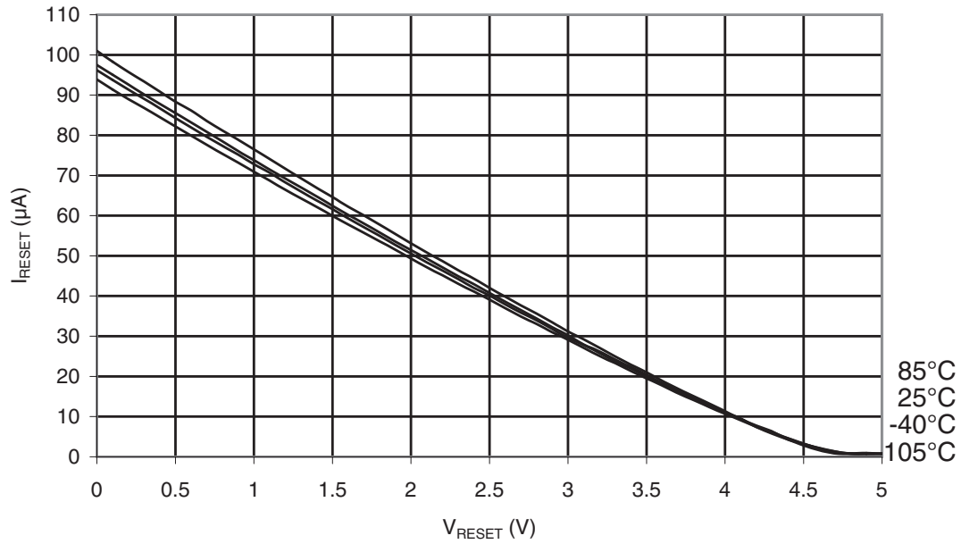
Figure 32-20. ATmega48PA: Reset Pull-up Resistor Current vs. Reset Pin Voltage ( V_{CC} = 5V )
