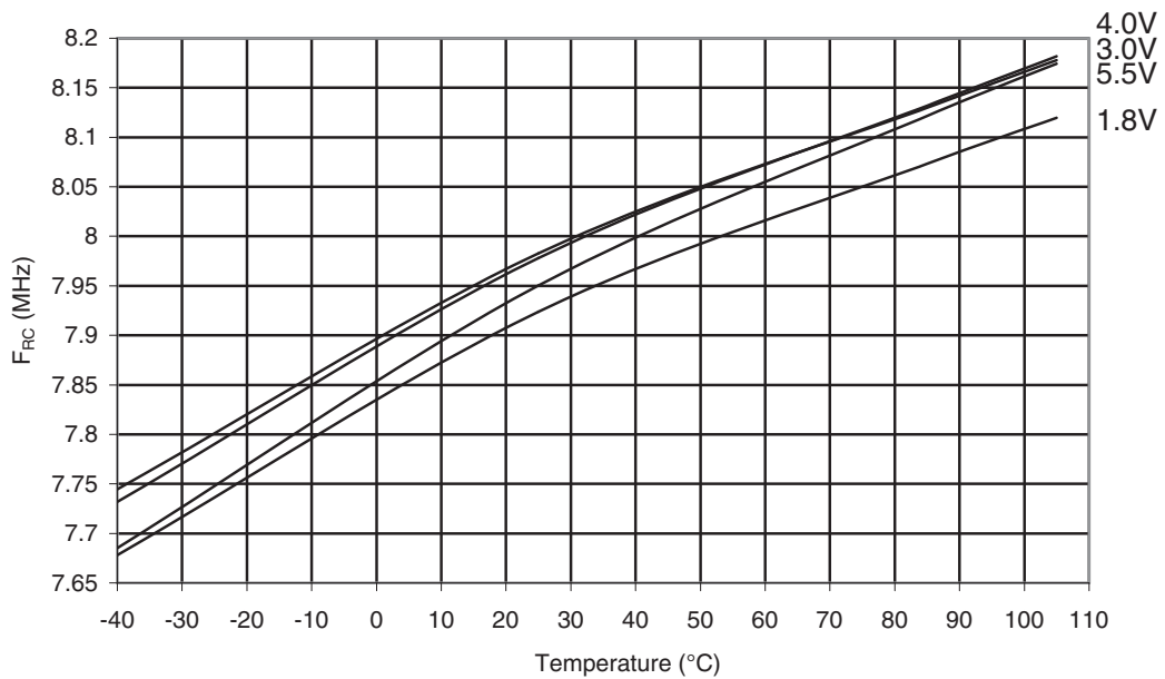
Figure 32-37. ATmega48PA: Calibrated 8MHz RC Oscillator Frequency vs. Temperature
