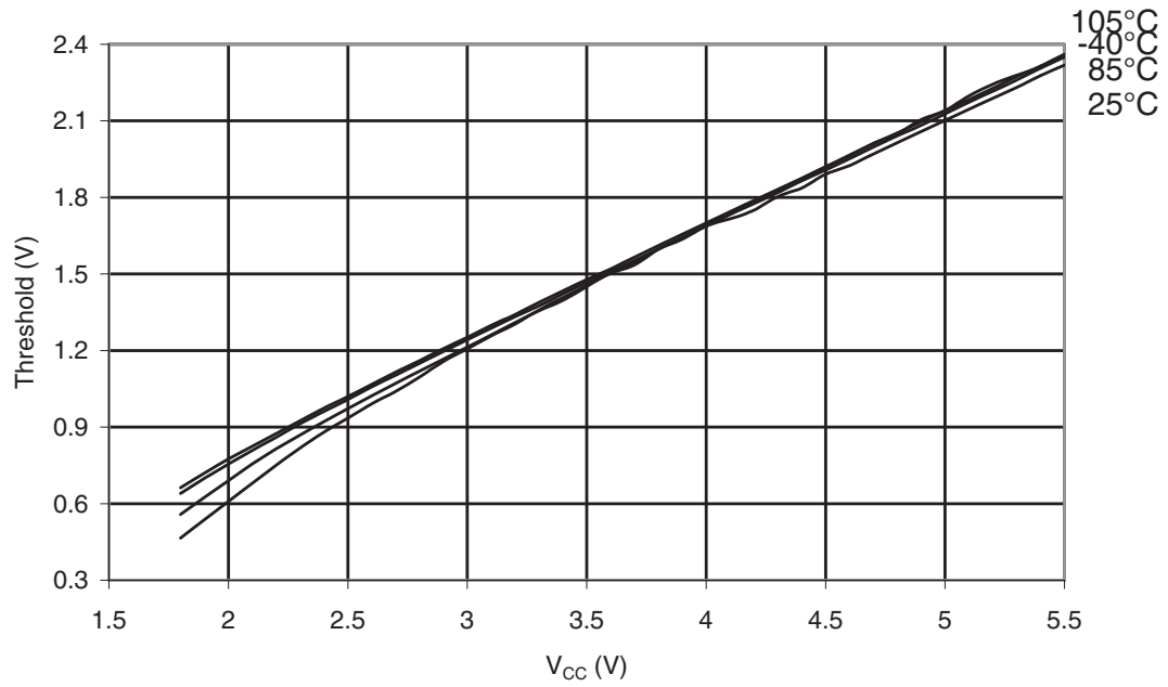
Figure 32-26. ATmega48PA: I/O Pin Input Threshold Voltage vs. V_{CC} ( V_{IL} , I/O Pin read as '0')
