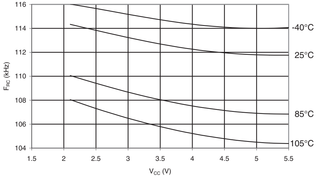
Figure 32-35. ATmega48PA: Watchdog Oscillator Frequency vs. V_{CC}
