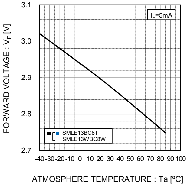
Fig.2-1 Forward Voltage - Atmosphere Temperature (BC8T, WBC8W)
