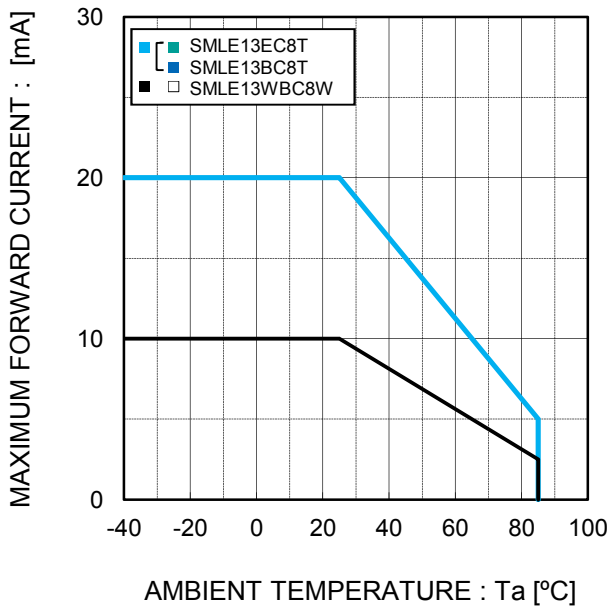
Fig.5 Derating
