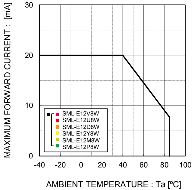
Fig.6 Derating
