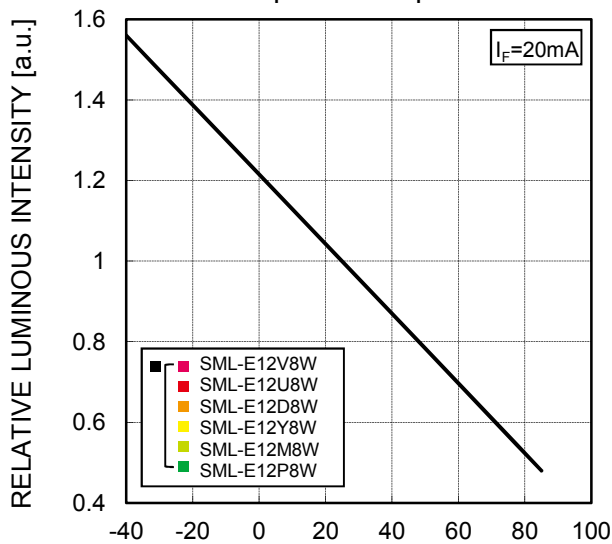
Fig.3 Luminous Intensity - Atmosphere Temperature
