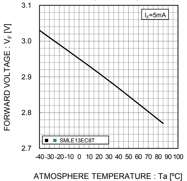
Fig.2-2 Forward Voltages - Atmosphere Temperature (EC8T)
