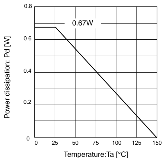
Figure 53. Power Dissipation (SOP-J8)
