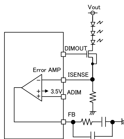
Figure 14. ISENSE pin circuit
