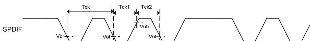
Figure VI.13.1 Timing chart
