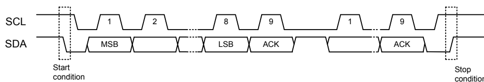
Figure VI.11.1 I 2 C start, stop condition
