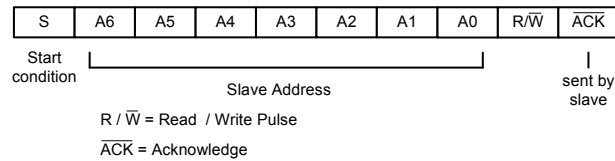
Figure VI.11.2 Slave Address Transfer Format
