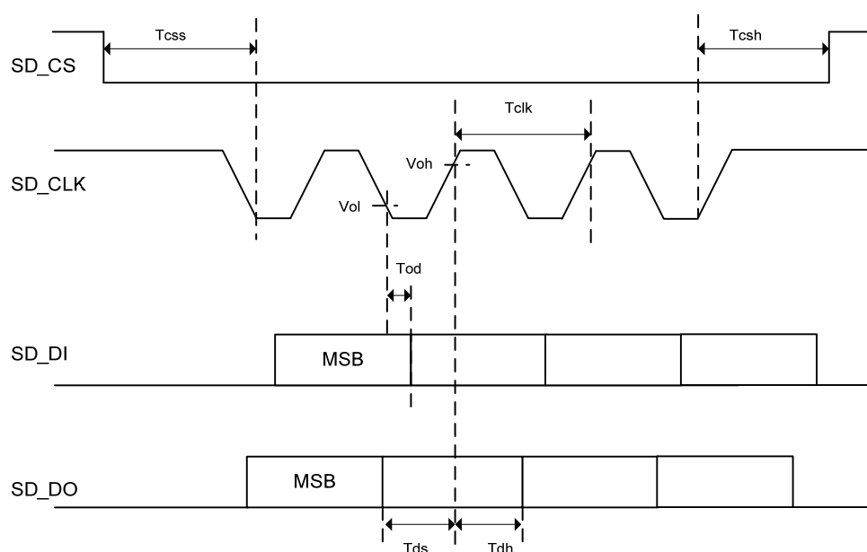
Figure VI.15.1 Timing chart of SPI for SD memory card
