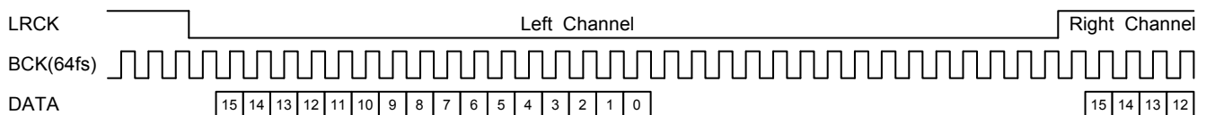
Figure VI.12.3 I 2 S Output Timing (64fs)
