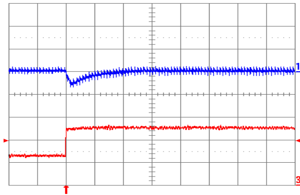
Fig. 1.8V.7: Output voltage response for V_{out} = 1.8 V to positive load current step change from 2.5 A to 5 A with slew rate of 5 A/ \mu s at V_{in} = 12 V. Top trace: output voltage (100 mV/div.); Bottom trace: load current (2 A/div.). C_o = 47 \mu F ceramic. Time scale: 20 \mu s/div.
