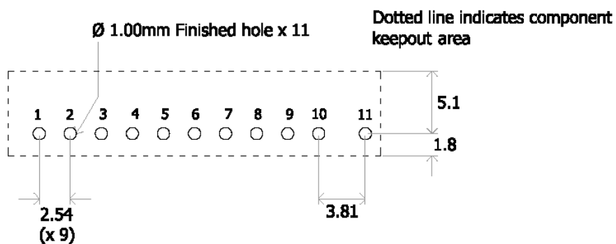
Figure 57. Recommended Footprint – Top View
