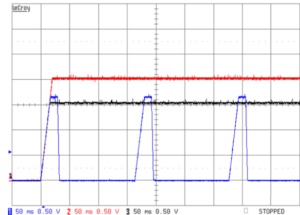
Figure 37. Turn-On into UVP on V3. The UV Fault Is Programmed To Be Non-Latching. Ch1 – Vo1, Ch2 – Vo2(Group A), Ch3 – Vo3 (Group B) Vo4 not shown.
