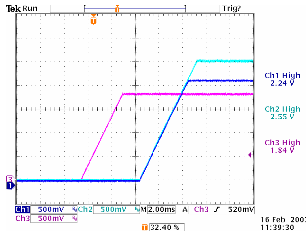
Figure 24 Two outputs delayed 5ms. All slew rates at 0.5V/ms.
