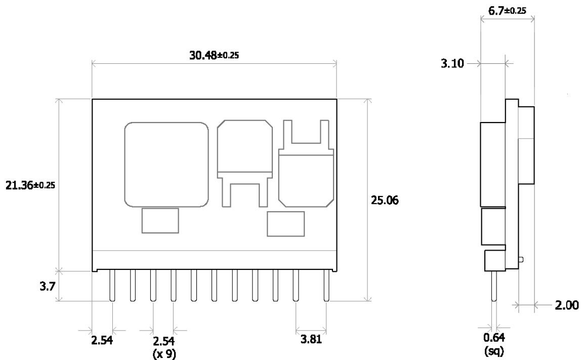
Figure 56. Mechanical Drawing
