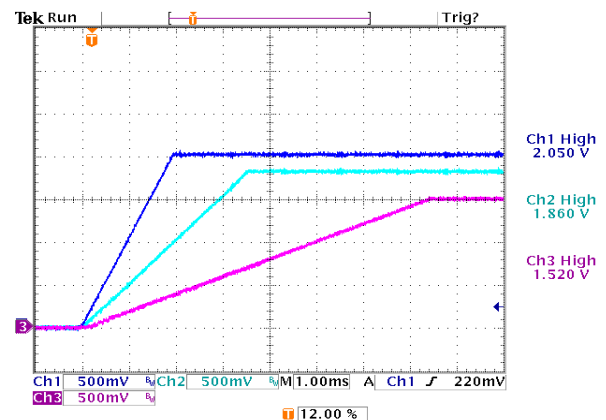
Figure 22. Turn-On with Different Rising Slew Rates. Rising Slew Rates are V1-1V/ms, V2-0.5V/ms, V3-0.2V/ms.
