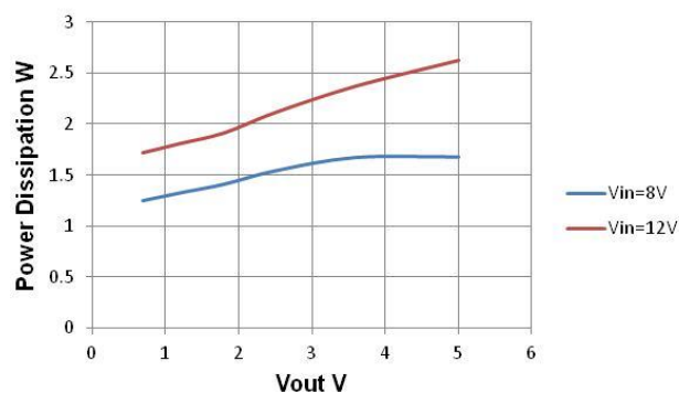
Figure 9. Power Dissipation vs V_{out} , I_{out}=5A , F_{sw}=500KHz
