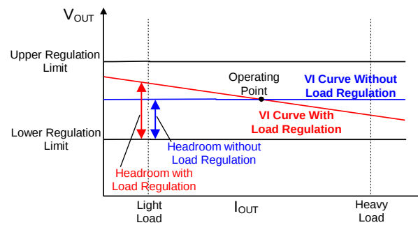
Figure 13. Optimal Voltage Positioning Concept
