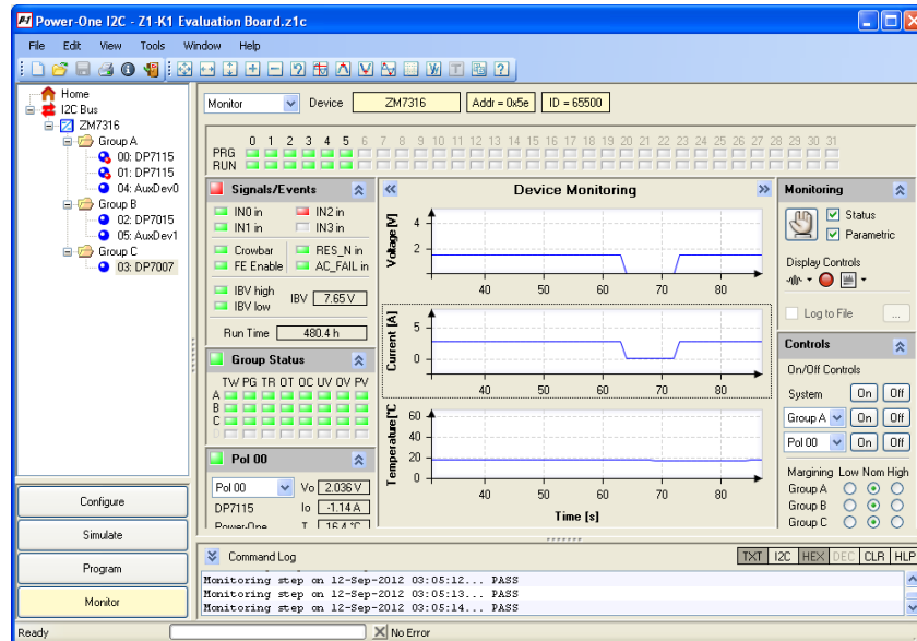
Figure 50. DPM Monitoring Window
