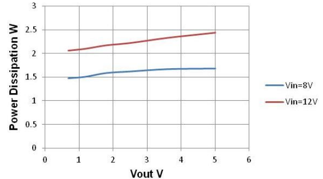
Figure 10. Power Dissipation vs V_{out} , I_{out}=5A , F_{sw}=1MHz
