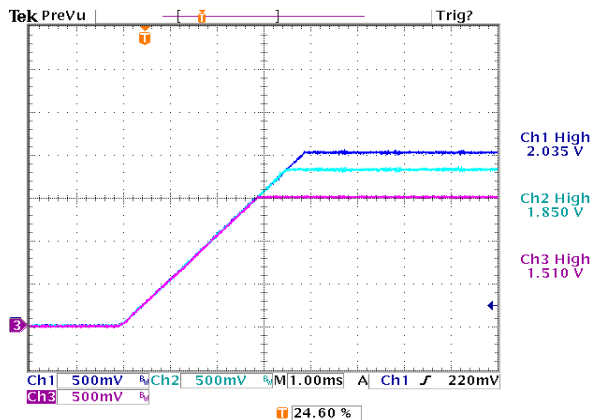
Figure 21. Tracking Turn-On. Rising Slew Rate is Programmed at 0.5V/ms for each output.
