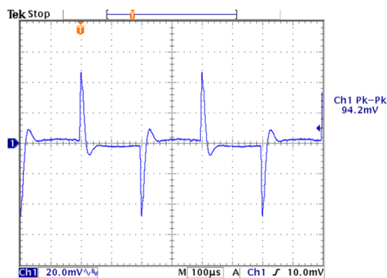
Figure 14 Transient Response with Regulation set to 0 mV/A.
