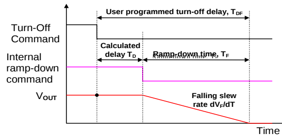
Figure 18. Relationship between Turn-Off Delay and Falling Slew Rate
