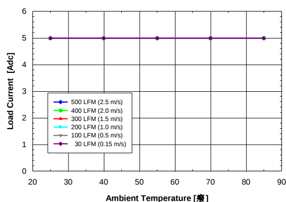
Figure 2. Available output current vs. ambient air temperature and airflow rates for converter DP8105G mounted horizontally with air flowing from input to output, MOSFET temperature \leq 120^{\circ}\text{C} , V_{in} = 12\text{ V} , V_{out} = 5\text{ V} , and F_{sw} = 1\text{MHz}
