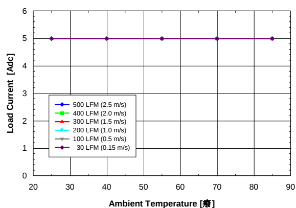
Figure 1. Available output current vs. ambient air temperature and airflow rates for converter DP8105G mounted horizontally with air flowing from input to output, MOSFET temperature \leq 120^{\circ}\text{C} , V_{in} = 12\text{ V} , V_{out} = 5\text{ V} , and F_{sw} = 500\text{KHz}
