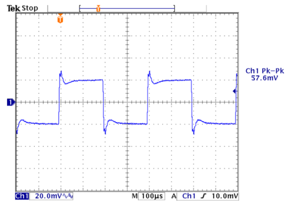
Figure 15 Transient response with non-zero Regulation.
