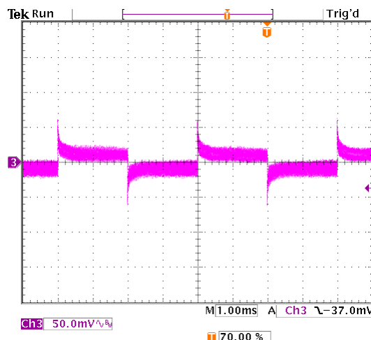
Figure 49. Transient Response with Regulation set to 6.53 mV/A
