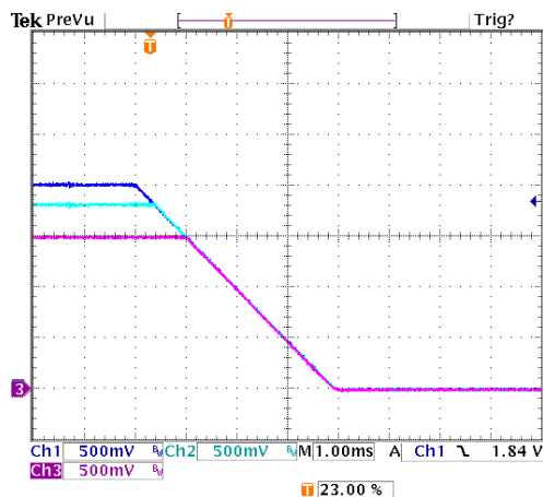
Figure 26. Tracking Turn-Off. Falling Slew Rate is Programmed at 0.5V/ms. Figure 27. Turn-Off with Tracking and Sequencing. Falling Slew Rate is Programmed at 0.5V/ms.
