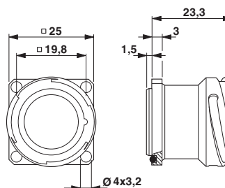
Dimensional drawing
