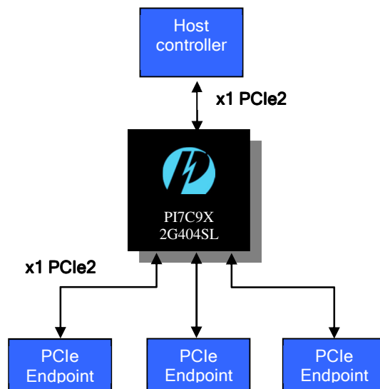
PI7C9X2G404SL – Application Example
