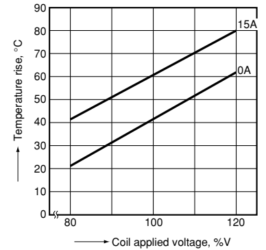
2-(4). Coil temperature rise (2 Form C/DC type)
