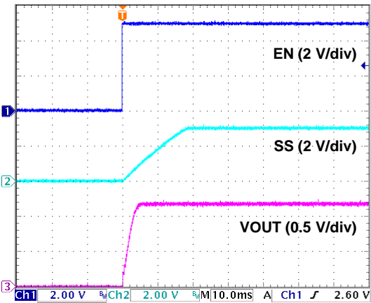
Time (10 ms/div)
