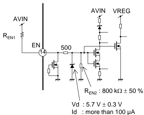
Figure : Internal circuit with EN pin
