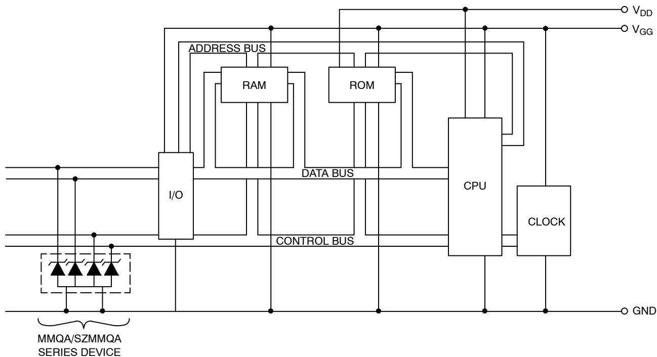
Figure 10. Microprocessor Protection
