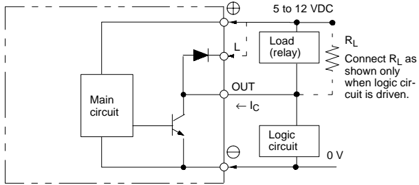
EE-SB5M(C) Light-ON/Dark-ON
