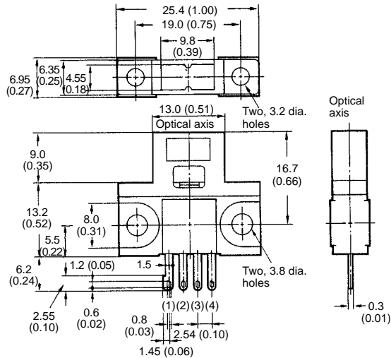
Terminal Arrangement
