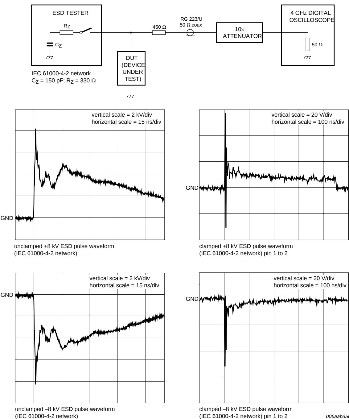
Fig 4. ESD clamping test setup and waveforms
