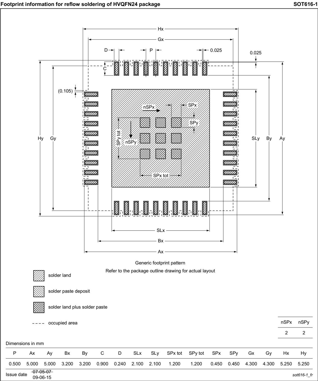
Fig 36. PCB footprint for SOT616-1 (HVQFN24); reflow soldering
