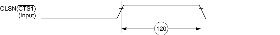
Figure 50. Ethernet Collision Timing Diagram
