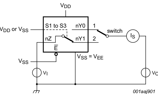
Fig 9. Test circuit for measuring OFF-state leakage current nYn port
