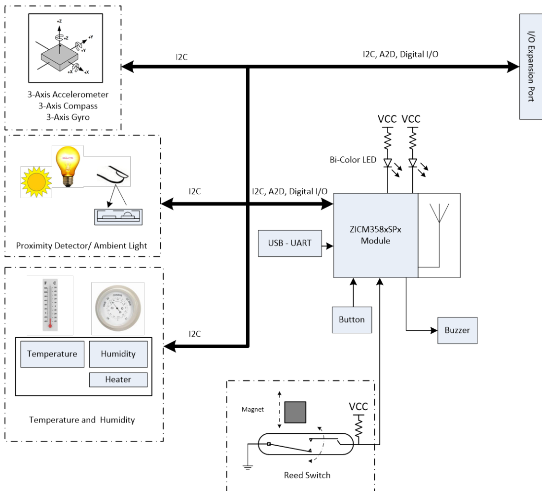
SENSOR NODE - Block Diagram
