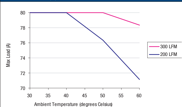
THERMAL DERATING GRAPH
