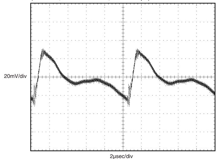
Output Ripple and Noise
