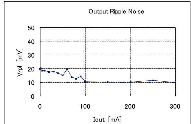
Vin=5.0V, Vout=3.3V, BW: 150MHz
