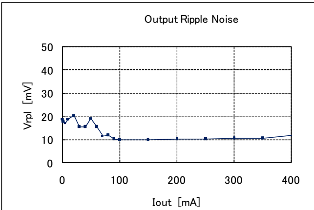
Vin=5.0V, Vout=3.0V, BW: 150MHz
