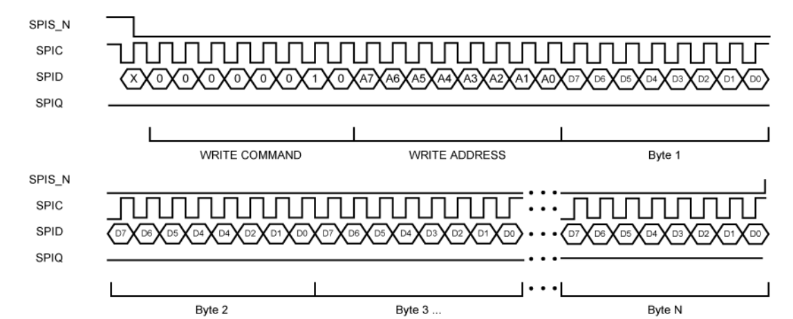
Figure 12. SPI Multiple Write
