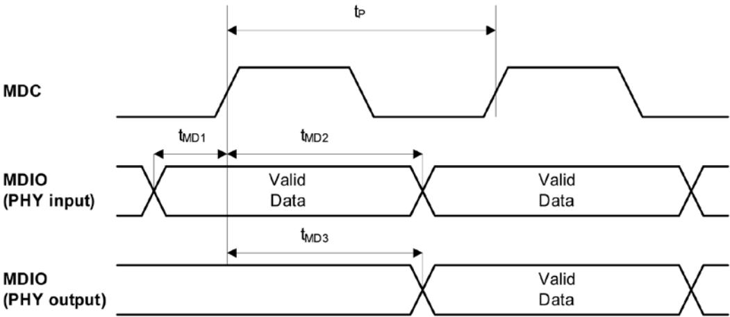
Figure 31. MDC/MDIO Timing
