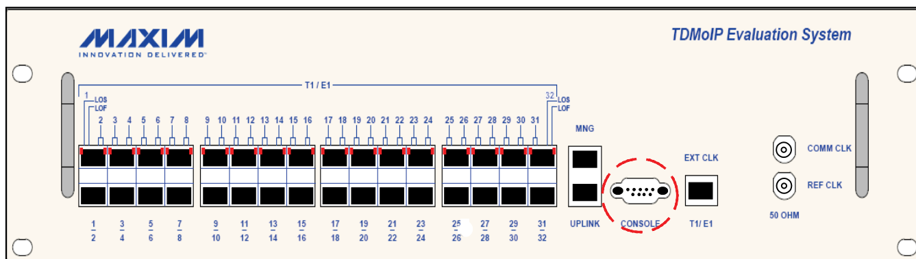
Figure 2-8. CONSOLE Connector
