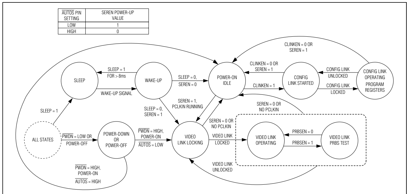
Figure 33. State Diagram, All Applications
