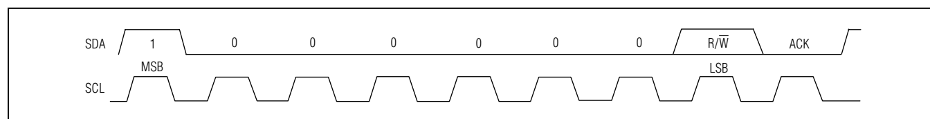
Figure 27. Slave Address
