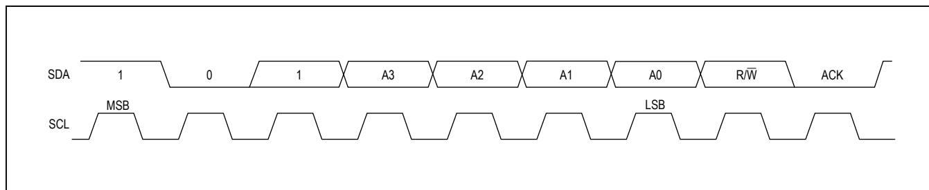
Figure 5. Slave Address
