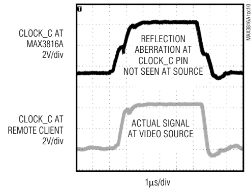
REFLECTION ABSORBED BY MAX3816A
