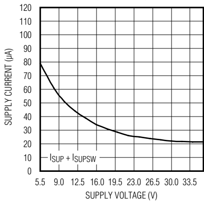
SUPPLY CURRENT vs. SUPPLY VOLTAGE (5V/2.2MHz)
