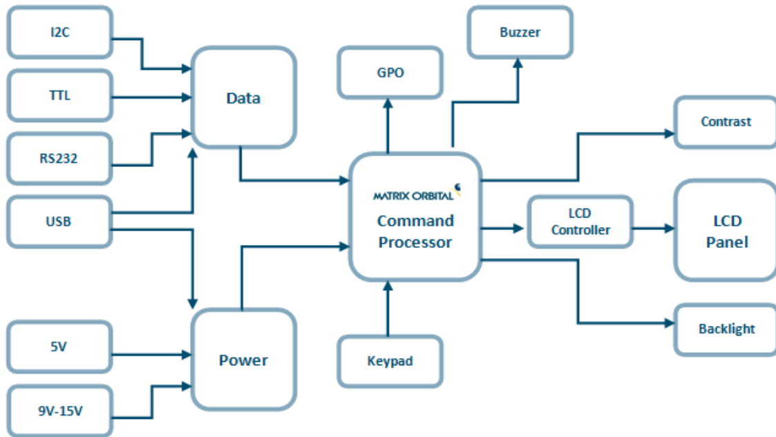
Figure 15: Functional Diagram
