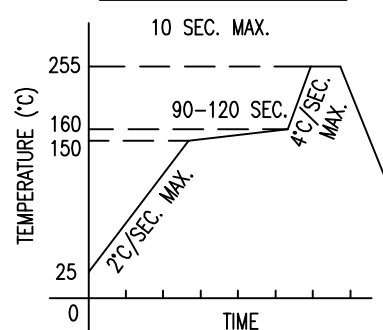
□ 0.30 [0.012] (2 PLS.) □ LEAD FREE REFLOW PROFILE
