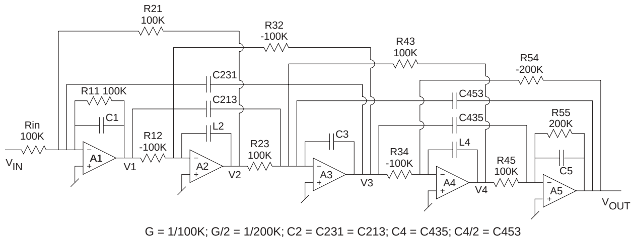
Figure 1. Simplified ispPAC80 Filter Core Schematic
