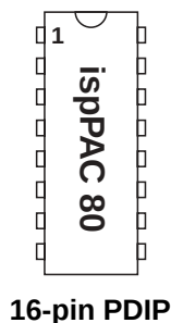
16-pin PDIP
